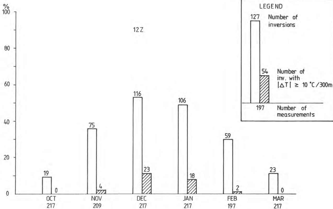
Fig 2. Statistics of inversions at Sundsvall/Härnösand aerodrome 1972-1978.
