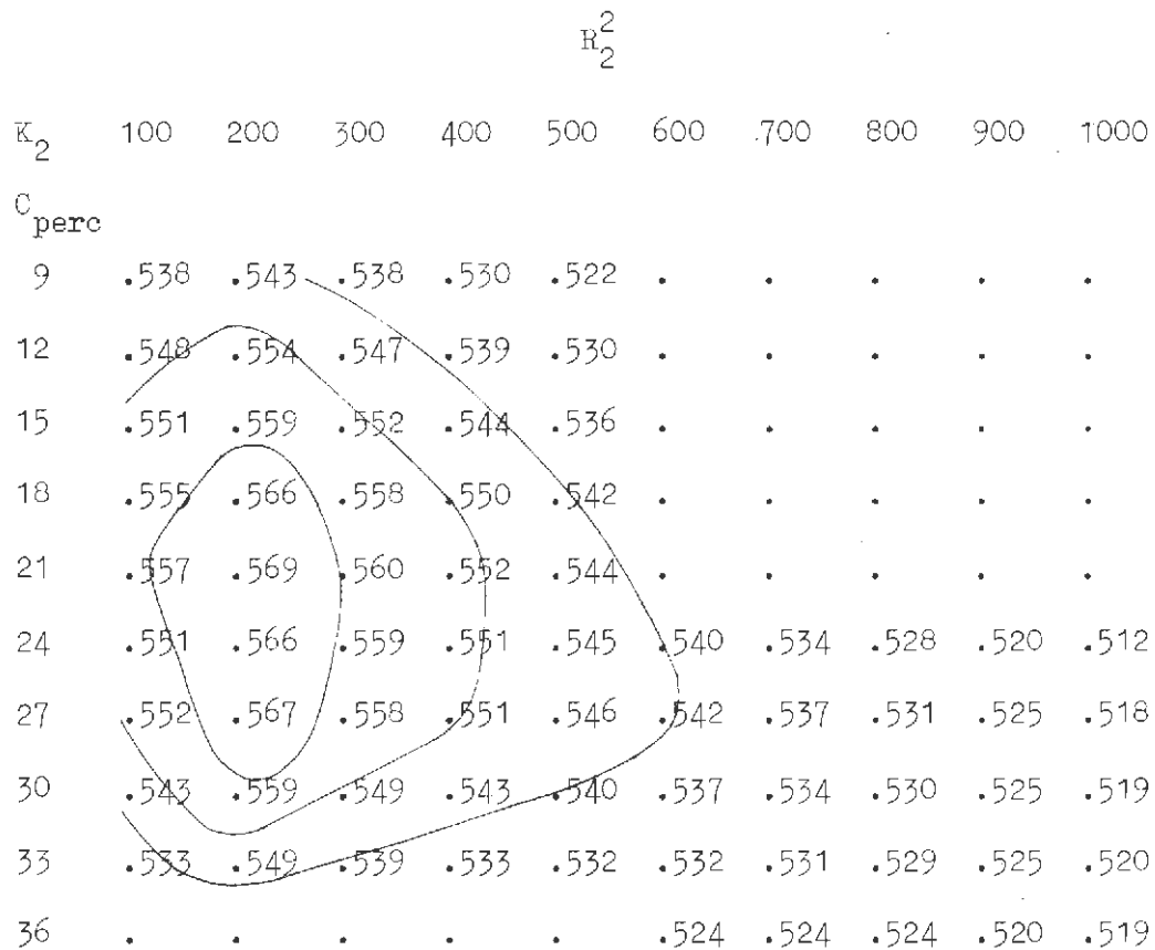
Fig. 5.3 The response of the R^2 -criteria to K_2 ( 1/(s \cdot mm) ) and C_{perc} ( 10^{-1} mm/day) at Kultsjön. (See chapter 5.3; 5.3.1)
