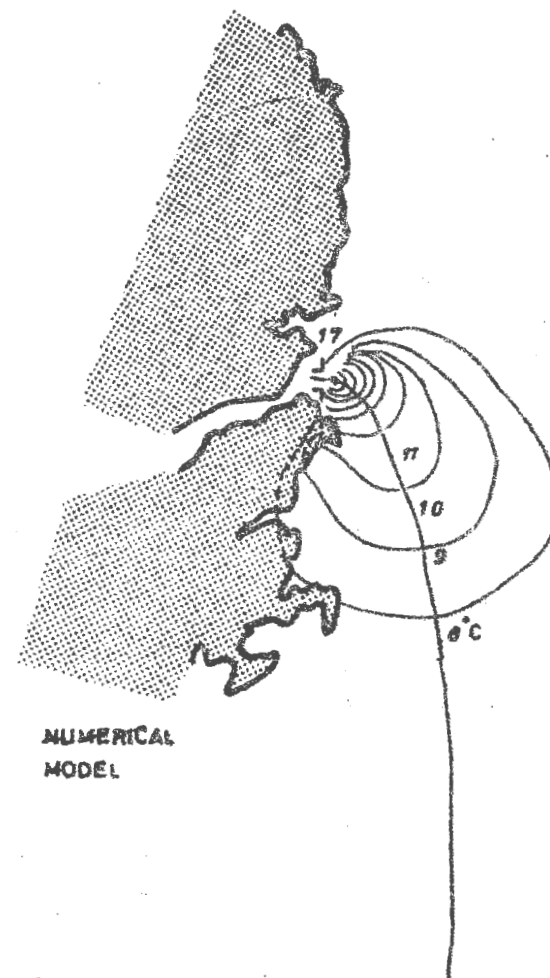
Figure 2.1 Direct comparison of isotherms, Case A
