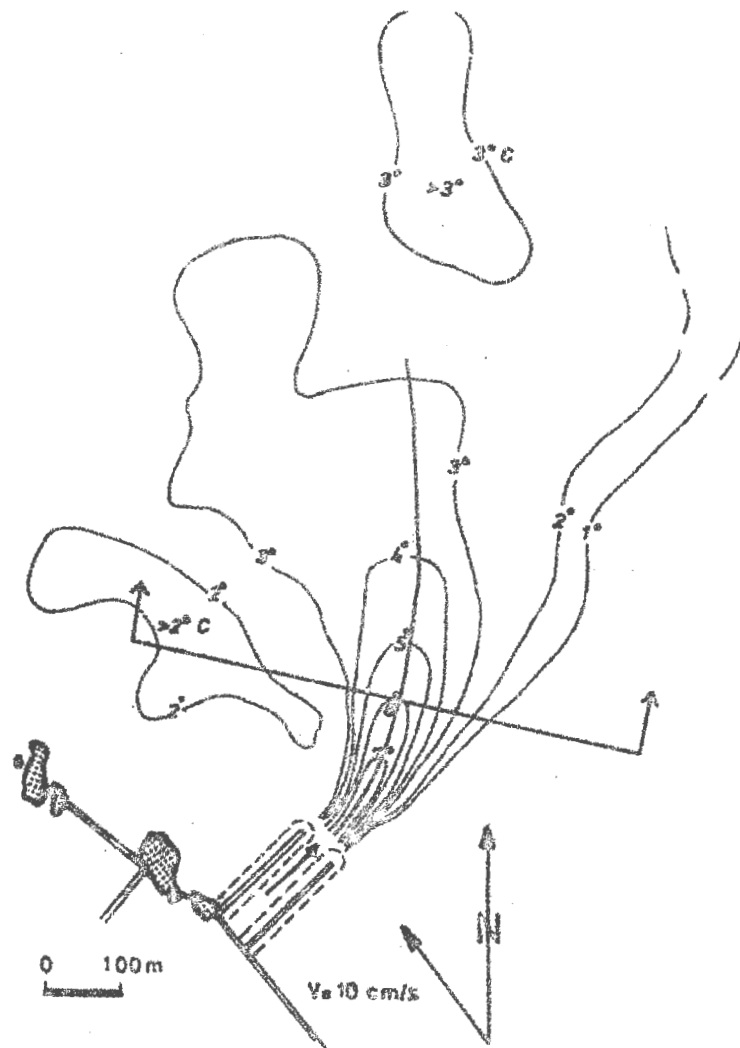
Figure 2.23 Forsmark Power Plant model temperatures
