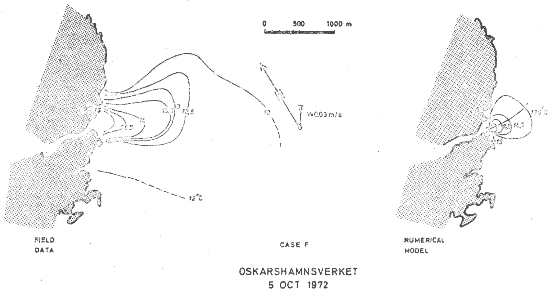
Figure 2.11 Direct comparison of isotherms, Case F
