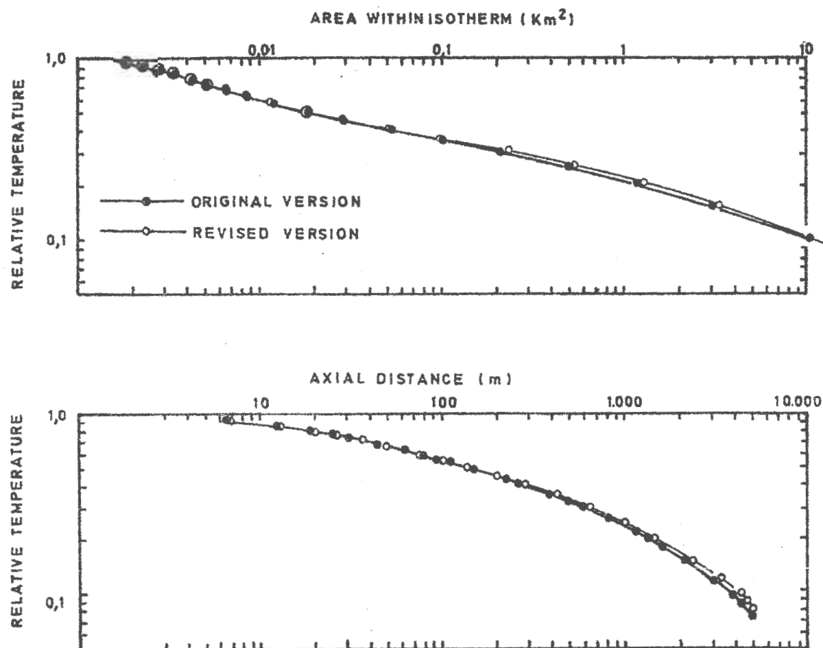
Figure 1.1 Effects of program revisions. Data for Oskarshamnsverket, restricted outlet, Q_0 = 22 \text{ m}^3/\text{s}
