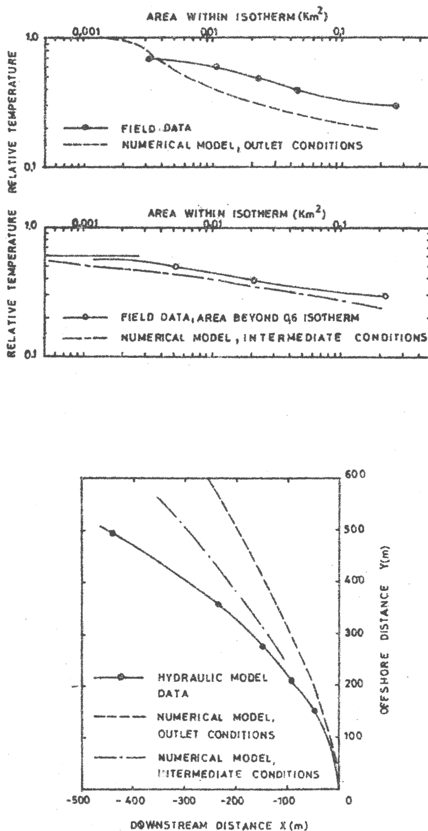
Figure 2.25 Comparison of enclosed areas and trajectory, Forsmark undistorted model
