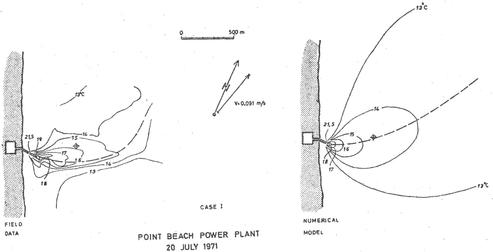
Figure 2.17 Direct comparison of isotherms, Case I
