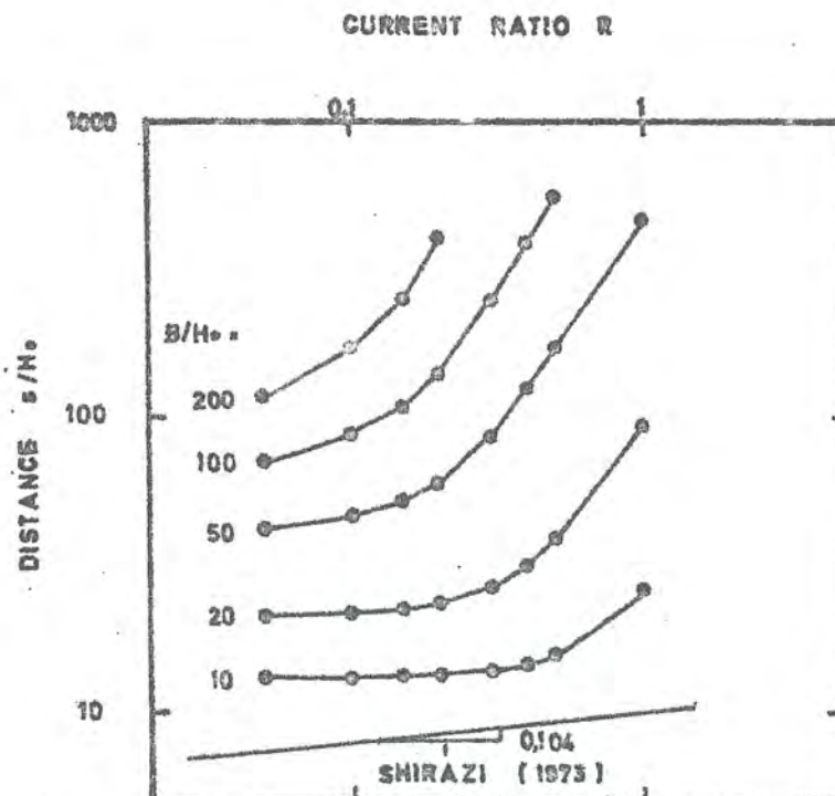
Figure 3.4 Effects of current strength on temperature and plume width, SMHiverket
