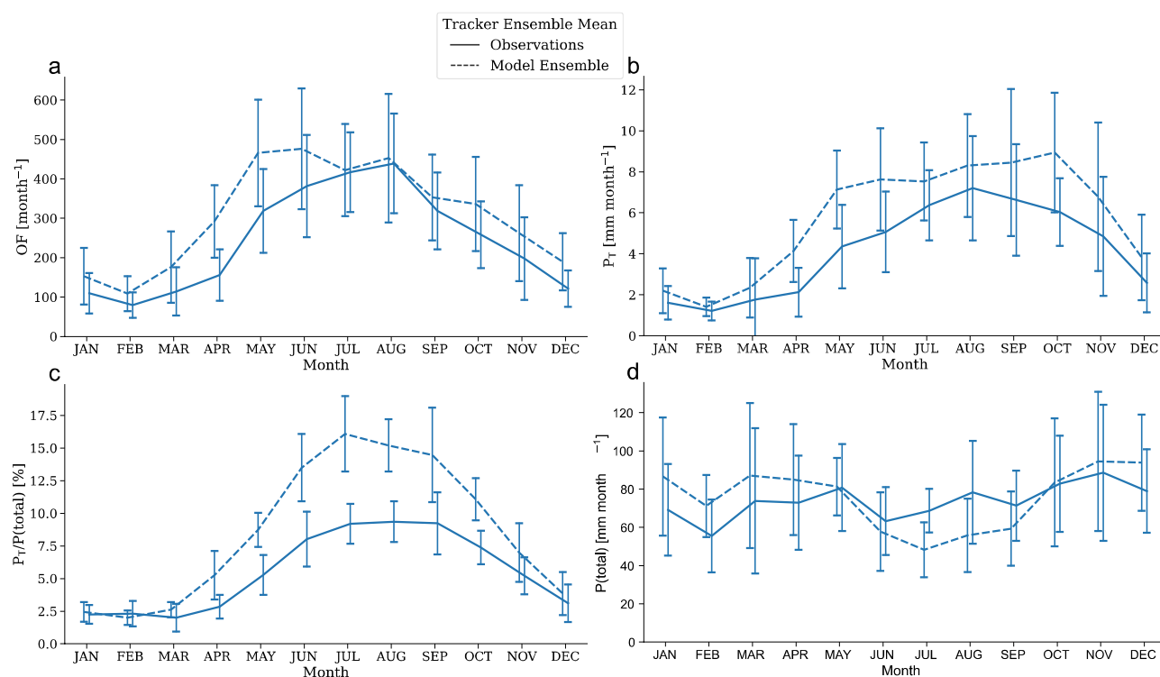
Fig. 4 Annual cycles for the tracker ensemble mean of both the model ensemble (dashed line) and observations (solid line), with panel a showing track occurrence frequency, OF [ \text{month}^{-1} ], panel b accumulated precipitation of tracks, P(tracks) [ \text{mm month}^{-1} ], panel c heavy precipitation fraction, P(tracks)/P(total) [%], and panel d accu-
