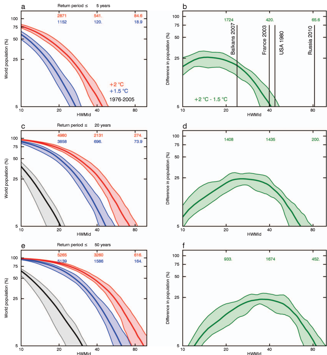
Figure 4. Fraction of world population exposed to heat waves. (a),(c),(e) Cumulative distribution function of global population (%) affected by heat waves with return period less than 5 (a), 20 (c) and 50 (e) years, respectively, for the reference period (black line), 1.5 °C world (blue) and 2 °C world (red). Results are shown as median and range (shading) of the model runs. Numbers indicate the absolute difference, compared to the reference period, in the number of people (in millions) exposed to severe (HWMId = 20), extreme (HWMId = 40) and exceptional (HWMId = 80) heat waves in a 1.5 °C world (blue) and 2 °C world (red). (b), (d), (f) Difference (%) between the number of people exposed to heat waves in the 1.5 °C world and 2 °C world. In (b), vertical lines indicate the magnitude of some observed heat waves. Numbers indicate the absolute difference (2 °C world vs. 1.5 °C world), in the number of people (in millions) exposed to severe, extreme, and exceptional heat waves.
