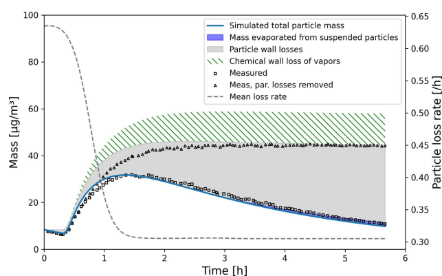
Figure 11. Comparison against \alpha -pinene oxidation experiment (exp. 13, Pathak et al., 2007). Size-resolved aerosol wall losses were measured for the same chamber in Pierce et al. (2008). Moderate chemical wall loss is calculated with parametrization from ARCA box using \text{ALPHAWALL} = 5 \times 10^{-5} , \text{CW\_EQV} = 40 \mu\text{m m}^{-3} and \text{EDDYK} = 0.05 \text{ s}^{-1} .
