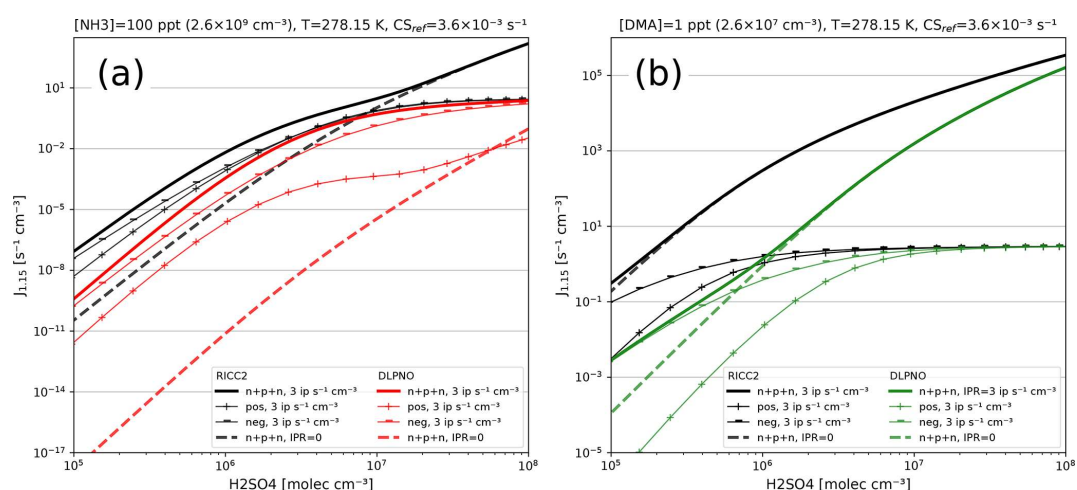
Figure 9. Steady-state particle formation rates from the two \text{H}_2\text{SO}_4 – \text{NH}_3 (a) and two \text{H}_2\text{SO}_4 –DMA systems (b). Both chemistries include data from RICC2 and DLPNO level of theories. Thick lines show the total formation rate, and solid lines are in the presence of ions and dashed lines without ions present. All simulations used the same temperature ( 5^\circ\text{C} ) and external cluster losses ( 3.6 \times 10^{-3} \text{ s}^{-1} ).
