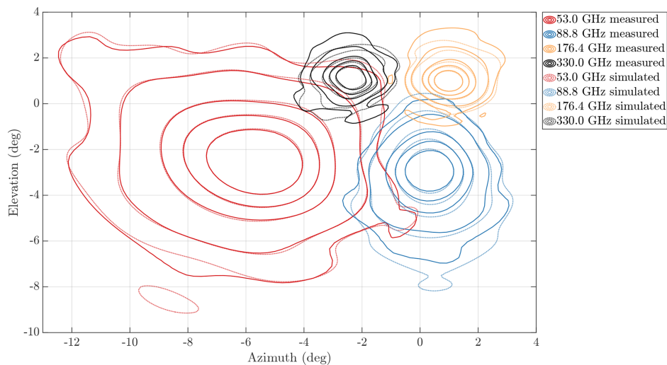
Figure 10. Comparison between measured (solid lines) and simulated (dotted lines) antenna responses, at 53.0 (red), 88.8 (blue), 176.4 (yellow), and 330.0 (black) GHz. The contours at -3 , -6 , -10 , -20 and -30 dB, with respect to peak responses, are shown.
