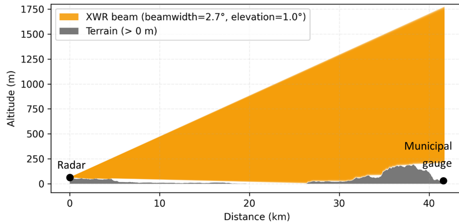
Figure 3. Elevation profile and beamwidth between the XWR radar location and the municipal gauge.
