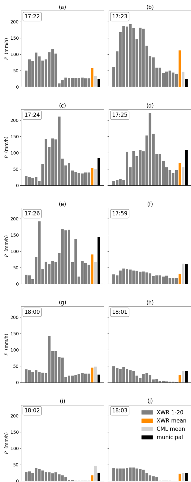
Figure 10. (a–e) Rainfall intensity 5 min before CML signal loss (17:22–17:26 UTC+2). (f–j) Rainfall intensity 5 min after signal loss (17:59–18:03 UTC+2). Twenty radar bins sampled along CML path every 250 m (XWR 1–20), XWR mean, CML mean and municipal gauge.
