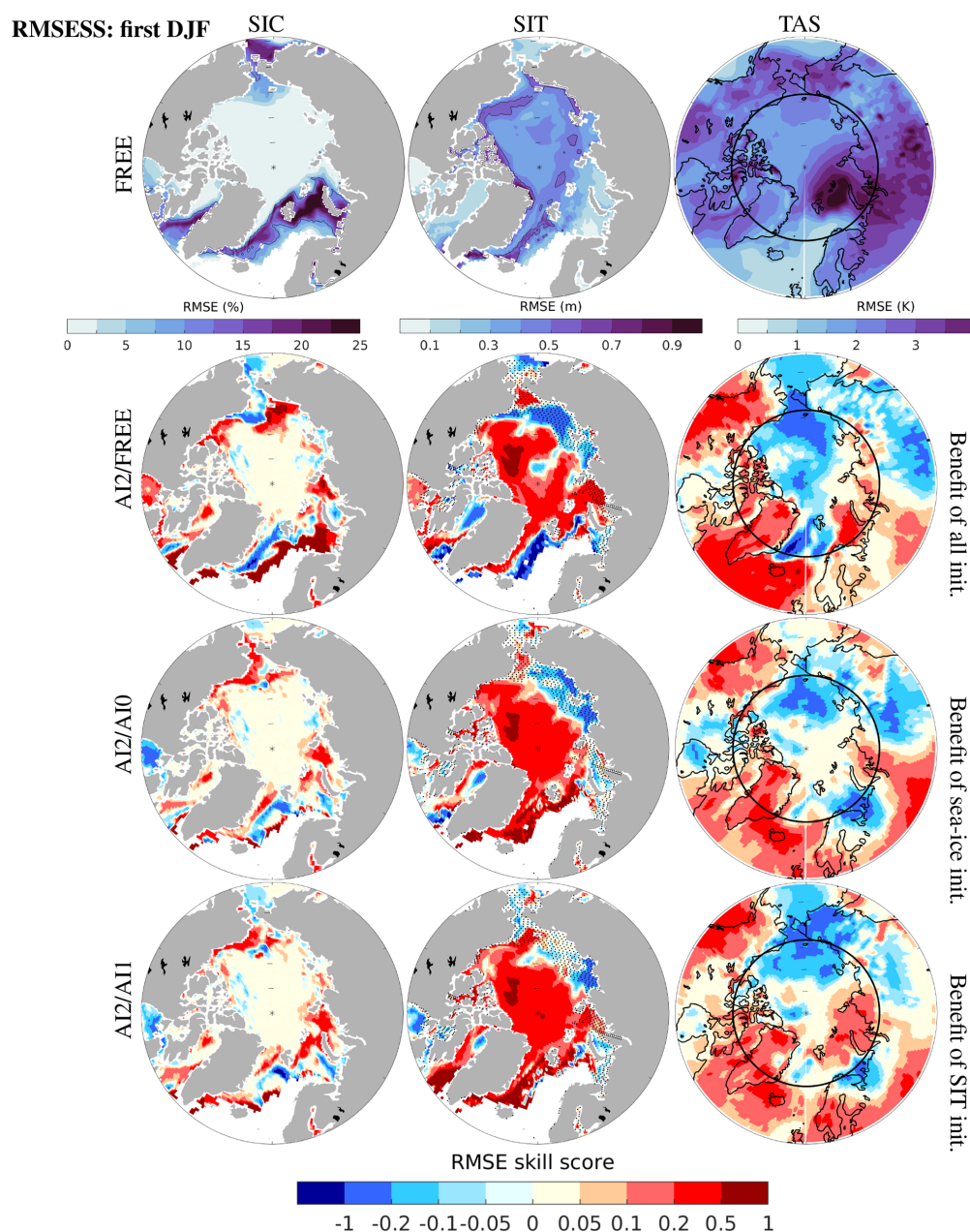
Figure 6. RMSE of FREE with respect to REF (top row) and RMSE skill score (lower rows) for the first wintertime (DJF) forecast: SIC (left), SIT (centre) and TAS (right). The contour lines mark \text{RMSE} \geq 10\% or 0.5\text{ m} for SIC and SIT, respectively. The RMSE skill score is calculated as 1 - (\text{RMSE}_{\text{AI2}}/\text{RMSE}_{\text{INIT}}) , where INIT denotes FREE (no init.), AI0 (no sea ice init.) and AI1 (no SIT init.). Scores above 0 denote more accurate in AI2 than INIT, and vice versa. Note that the label of the colour bar for skill score is asymmetric because the minimum of the skill score (SS) can be far below -1 in contrast to the maximum of 1. The stippled areas in the middle columns are the same as in Fig. 2b.
