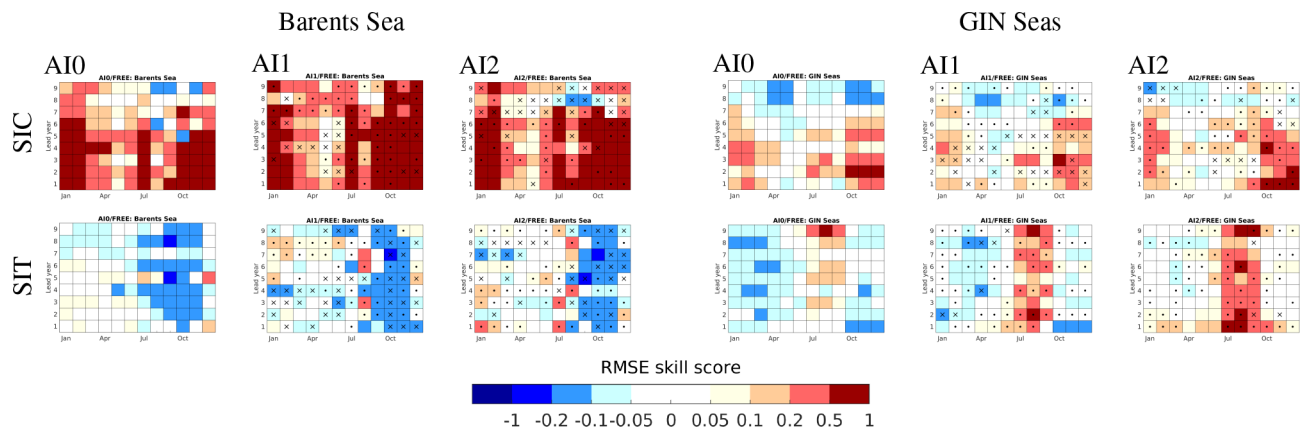
Figure 10. Regional Arctic SIC (upper) and SIT (lower) prediction in the Atlantic Arctic sector, i.e. Barents Sea (left) and GIN seas (right): RMSE skill score of AI0 / FREE, AI1 / FREE and AI2 / FREE, respectively. AI0 / FREE is calculated as 1 - (\text{RMSE}_{\text{AI0}} / \text{RMSE}_{\text{FREE}}) , where the ratio of RMSE is averaged over regions. Scores above 0 denote more accurate in AI0 than FREE (red), and vice versa (blue). White colours denote a 0 score, which means RMSEs in AI0 (or AI1, AI2) and FREE are equal, respectively. Boxes for AI1 / FREE and AI2 / FREE are stippled by dots (or crosses) if the added skill is above 0.05 (or below -0.05 ), which is the minimal colour interval of RMSESS. The added skill is calculated for AI1 as (\text{AI1} / \text{FREE} - \text{AI0} / \text{FREE}) and for AI2 as (\text{AI2} / \text{FREE} - \text{AI1} / \text{FREE}) , respectively.
