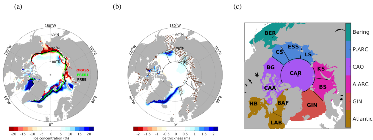
Figure 2. Model bias with respect to ORAS5 (REF) on 1 November for the period 1979–2014 for the single-member FREE1. (a) SIC. Colour lines indicate the September sea ice extent (15 % SIC) climatology for ORAS5 (red), FREE1 (green) and FREE (black). (b) SIT with dots indicating a mask for area with water depth < 100 m where no SIT initialization is applied. The maps have the bounding latitude at 56° N. Blue areas represent regions with more SIC and SIT in the model than REF, reflecting cold bias in surface temperature. (c) Regions considered for Arctic sea ice. Atlantic MIZ (brown): Hudson Bay (HB), Baffin Bay (BAF) and the Labrador Sea (LAB); the GIN seas (red); Atlantic Arctic (pink): Barents Sea (BS) and Kara Sea (KS); central Arctic Ocean (CAO, purple): central Arctic (CAR, 80° N north), Canadian Archipelago (CAA) and Beaufort Gyre (BG); Pacific Arctic (blue): Laptev Sea (LS), East Siberian Sea (ESS) and Chukchi Sea (CS); Bering Sea (BER, green).
