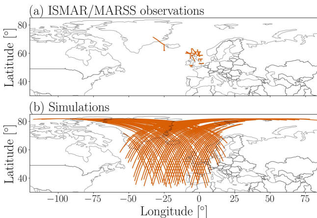
Figure 4. Locations of observations from the ISMAR and MARSS flight campaigns are displayed in panel (a), using cases where flight altitude was greater than 9 km. Locations of the simulated ISMAR and MARSS observations are displayed in panel (b).
