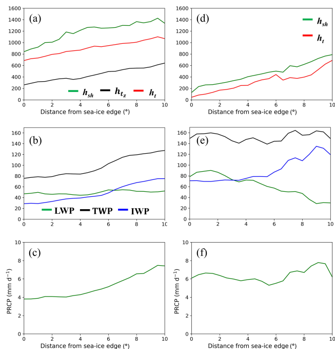
Figure 9. Average variation of (a) the height to the maximum specific humidity ( h_{sh} ), temperature gradient ( h_{tz} ; m), and temperature ( h_t ); (b) liquid water path (LWP; \text{g m}^{-2} ), ice water path (IWP; \text{g m}^{-2} ), and total water path (TWP; \text{g m}^{-2} ); (c) precipitation rate (PRCP; \text{mm d}^{-1} ), with the downstream northward distance from sea-ice edge, along the WaMAI trajectories over the Barents Sea. Panels (d), (e), and (f) are the counterparts of panels (a), (b), and (c) over the frozen seas. Note that this is not necessarily the distance traveled, since WaMAIs do not need to travel due northward.
