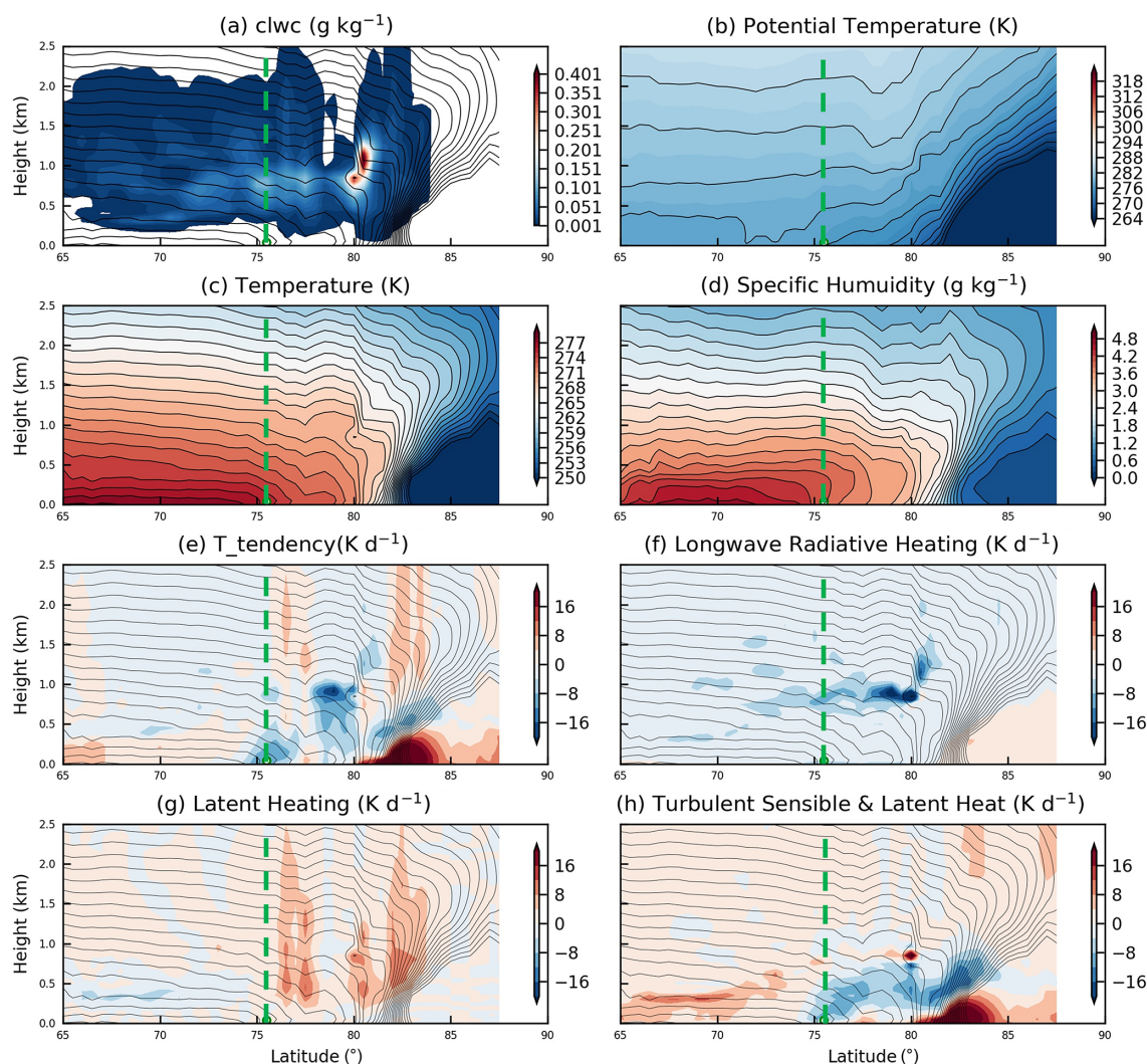
Figure 14. Same as Fig. 11 but for a selected turbulence-dominated WaMAI with cold dome.
