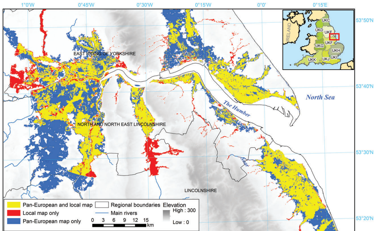
FIGURE 4 An example of the differences between the pan-European map from this study and the local reference map, for the Humber river estuary in England, both for the 100-year flood scenario (Environment Agency 2016)
