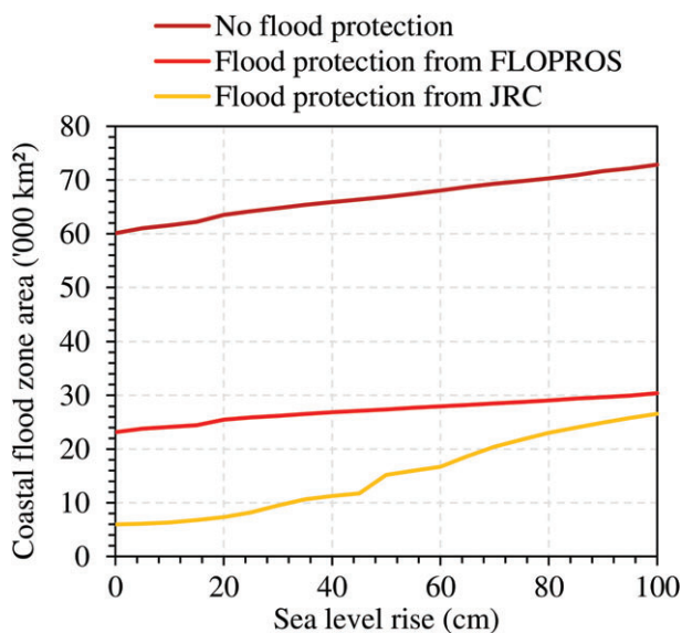
FIGURE 7 100-year coastal flood zone area in Europe (EU plus Norway) assuming uniform sea level rise and using different assumptions of flood protection
