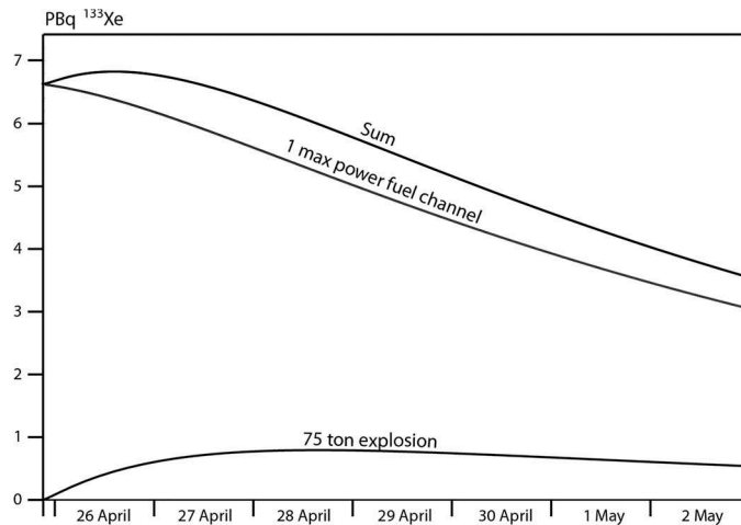
Fig. 3. The development of the 133 Xe activity in the mass corresponding to one maximum power fuel channel with an internal 75-ton explosion ("Sum") and its two components: core and nuclear explosion.
