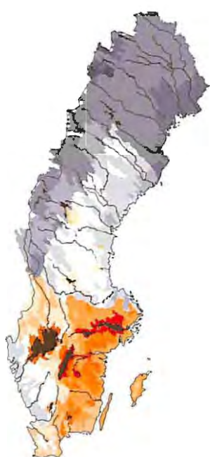
RCAO-HadAM3H-A2
