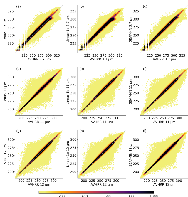
Figure 4. Radiance inter-comparisons for AVHRR channel 3B (3.7 \mu\text{m} , a–c ), channel 4 (11 \mu\text{m} , d–f ), and channel 5 (12 \mu\text{m} , g–i ). The figure shows merged results for all daytime categories. Original AVHRR vs VIIRS brightness temperatures (K) are shown in ( a ), ( d ), and ( g ). AVHRR vs VIIRS-simulated brightness temperatures are shown in ( b ), ( e ), ( f ), ( h ), and ( i ). ( b ), ( e ) and ( h ) show results from the Linear-1b method, while ( c ), ( f ), and ( i ) show simulated results from the SBA-NN method.
