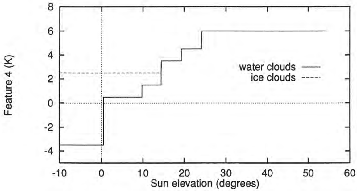
Figure 2. Feature 4 thresholds (temperature differences) as a function of sun elevations for the separation of all clouds from cloud-free surfaces during daytime and for the separation of water and ice clouds from cloud-free surfaces during night.
