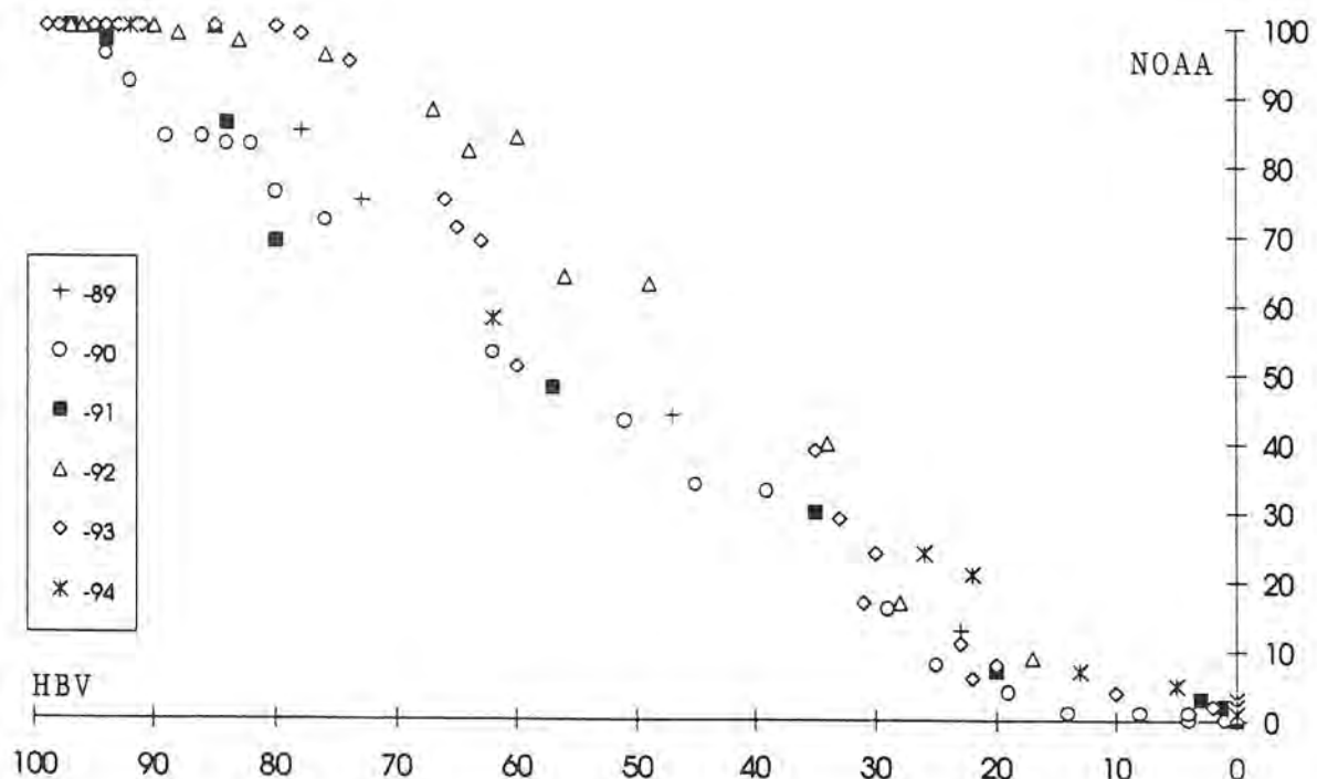
Figure 13. Modelled snow magazine (HBV - in percent of the maximum snow magazine) compared to SCANDIA-estimated snow area extent (NOAA) for the years 1989-1994 in the Suorva catchment area.
