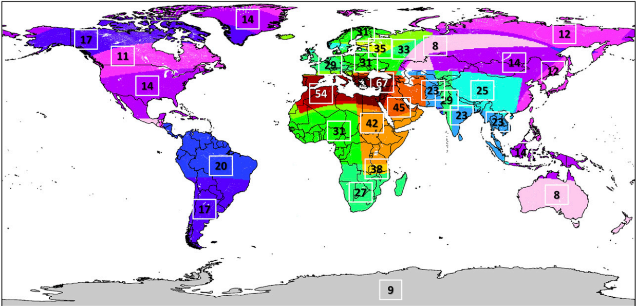
FIG. 1. Number of CORDEX simulations used. The numbers are valid for both RCP4.5 and RCP8.5.
