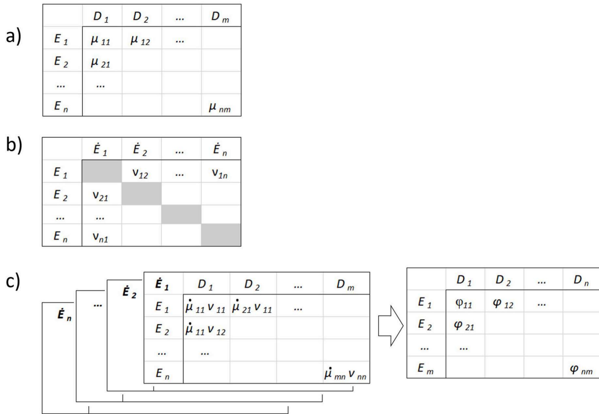
Fig. 1. Sensitivity matrices for total cumulative effects, where E are ecosystem components, D pressures and \mu , \nu , and \varphi are impact weights (shaded cells are not used). a) Original sensitivity matrix, b) sensitivity matrix incorporating ECIs, and c) a three-dimensional sensitivity matrix enabling indirect effects through other ecosystem components. The matrices to the left (calculation 1) transform into the matrix on the right (calculation 2) according to equations (4) and (5).
