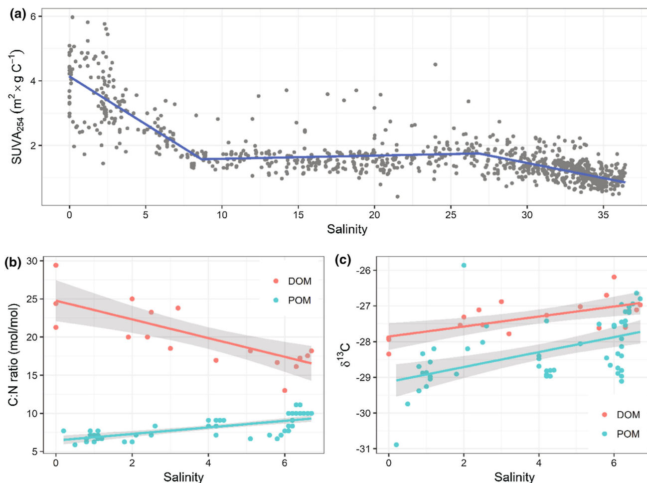
Fig. 6 Changing organic matter characteristics along the salinity gradient: a DOC-specific UV absorbance ( \text{SUVA}_{254} ), b C:N ratio and c stable isotope \delta^{13}\text{C} values in dissolved and particulate organic matter pools. Redrawn from Massicotte et al. (2017) (a), and Jilbert et al. 2018 (b, c)
