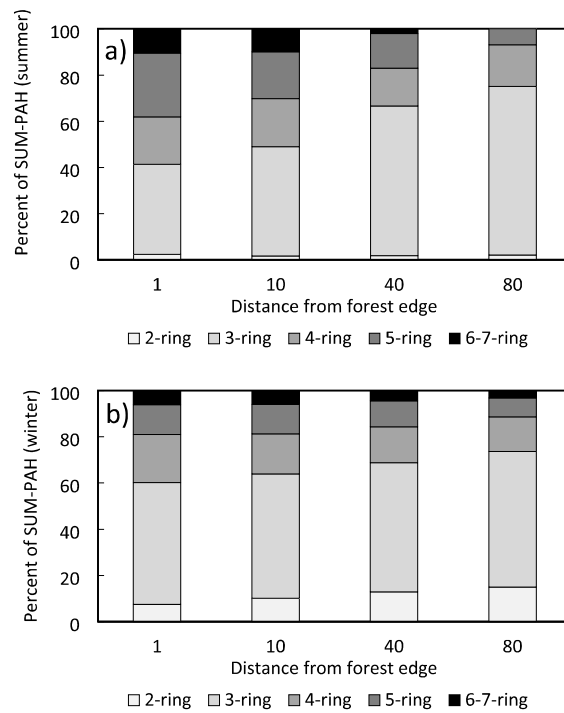
Fig. 5 Percentage of total SUM-PAH that consists of PAHs with different numbers of benzene rings during the approximately 4-week long summer (a) and winter (b) measurement periods at different distances from the edge of the spruce stand
