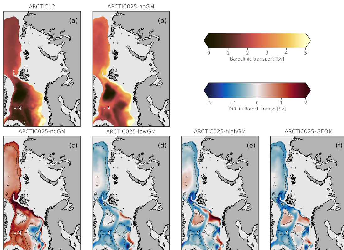
Figure 7. Panels (a) and (b) show the baroclinic transport function in ARCTIC12 and ARCTIC025-noGM, respectively. Panel (c) shows the difference between ARCTIC025-noGM and ARCTIC12. Panels (d)–(f) differences ARCTIC025-lowGM, ARCTIC025-highGM and ARCTIC025-GEOM relative to ARCTIC025-noGM. Note that regions shallower than the integration depth of 854 m has been masked out.
