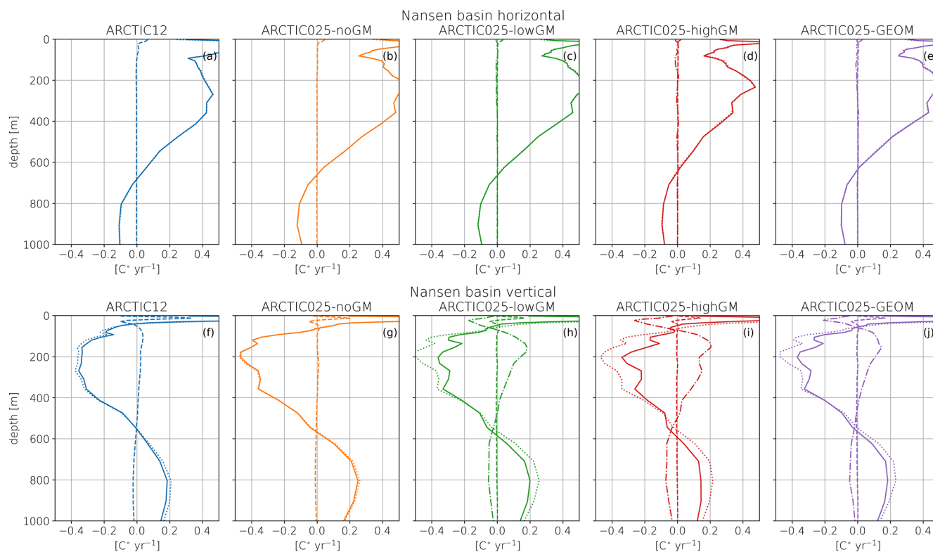
Figure B2. Time-mean (2008–2017) vertical profiles of horizontally averaged (over the Nansen basin) heat trend terms for advection (solid) decomposed into mean (dotted), resolved eddy (dashed), and parameterized eddy (dashed-dotted) contributions for each experiment. The upper row (a–e) shows horizontal, and lower row (f–j) vertical components.
