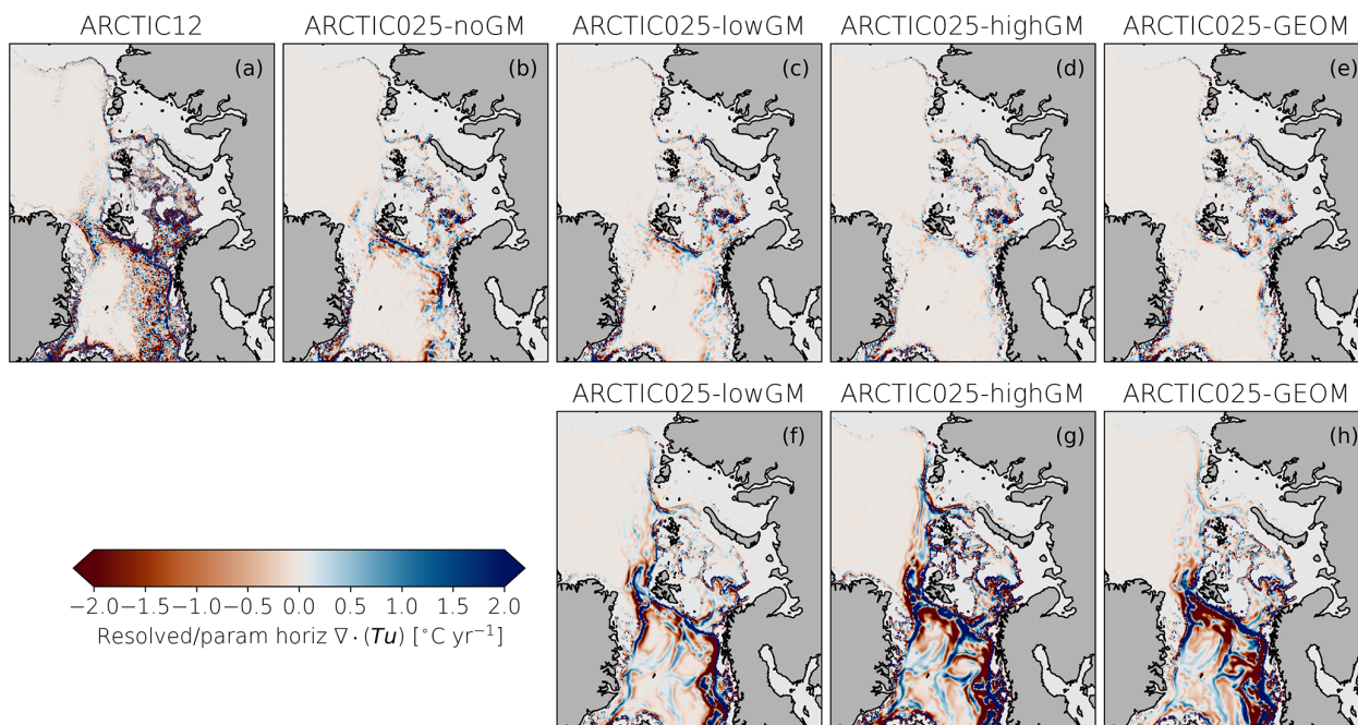
Figure 11. Horizontal component of the time-mean (2008–2017) divergence of resolved and parameterized eddy temperature fluxes in the Atlantic Water layer (233 m depth) for the different experiments.
