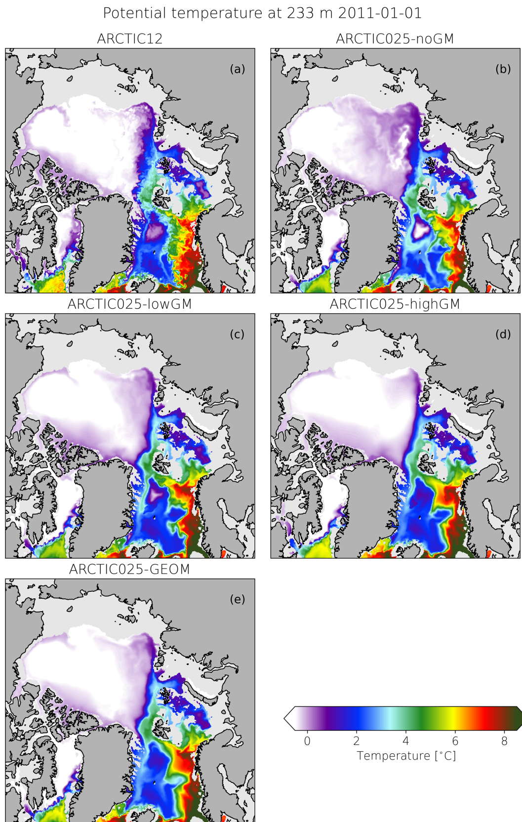
Figure A2. Daily snapshot (1 January 2011) of potential temperature in the Atlantic Water layer (233 m depth) computed for the different experiments.
