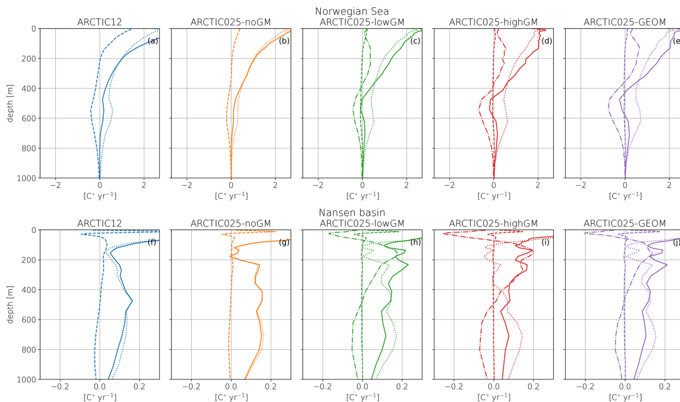
Figure 13. Time-mean (2008–2017) vertical profiles of horizontally averaged heat trend terms for total advection (solid) decomposed into mean (dotted), resolved eddy (dashed), and parameterized eddy (dashed-dotted) contributions for each experiment.
