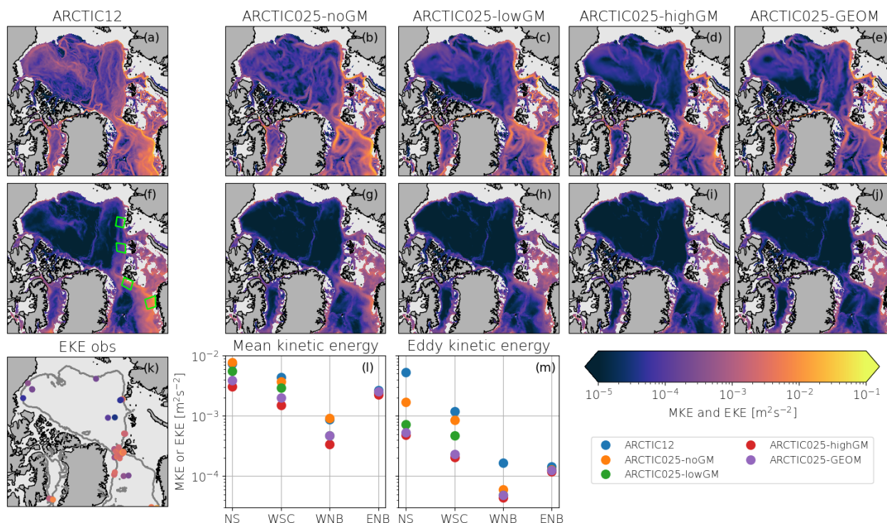
Figure 4. Panels (a)–(e) show the time-mean (2008–2017) MKE and panels (f)–(j) the EKE in the Atlantic Water layer (233 m depth) for the ARCTIC12, ARCTIC025-noGM, ARCTIC025-lowGM, ARCTIC025-highGM, and ARCTIC025-GEOM, respectively. Panel (k) shows observations of EKE from von Appen et al. (2022), averaged over the depth range 500–1000 m, with the grey line showing the 233 m isobath. Panels (l) and (m) show spatial averages of MKE and EKE at selected regions (green boxes in f) along the Atlantic Water pathway. The regions are NS = Norwegian Sea, WSC = West Spitzbergen Current, WNB = Western Nansen Basin, and ENB = Eastern Nansen Basin.
