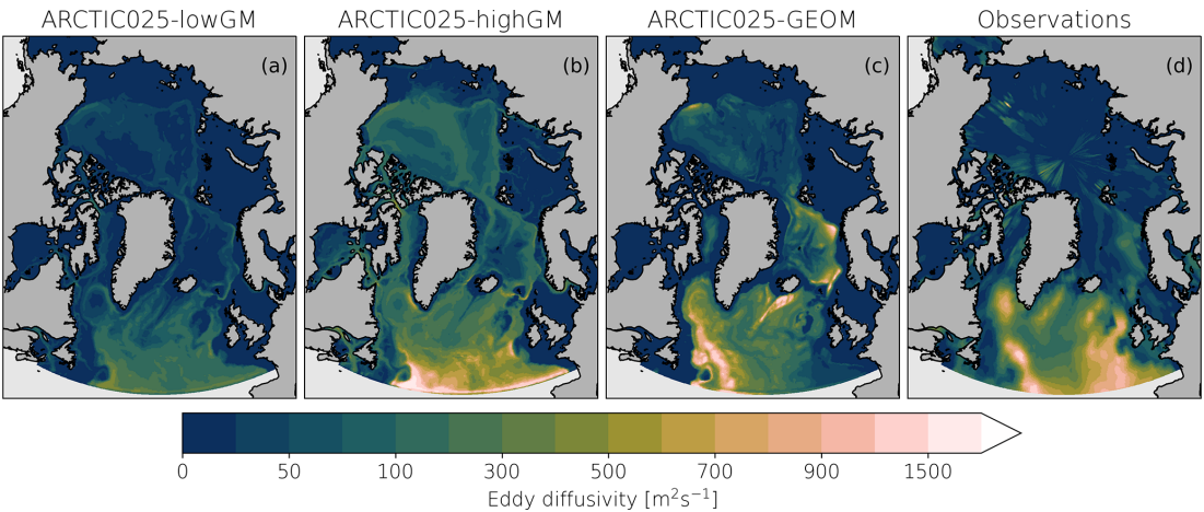
Figure 3. The time-mean (2007–2017) \kappa_{\text{GM}} fields for the (a) ARCTIC025-lowGM, (b) ARCTIC025-highGM, (c) ARCTIC025-GEOM, and d) observational estimate of surface \kappa_{\text{GM}} (Kusters et al., 2025). Note that the color range increases with increasing \kappa_{\text{GM}} .
