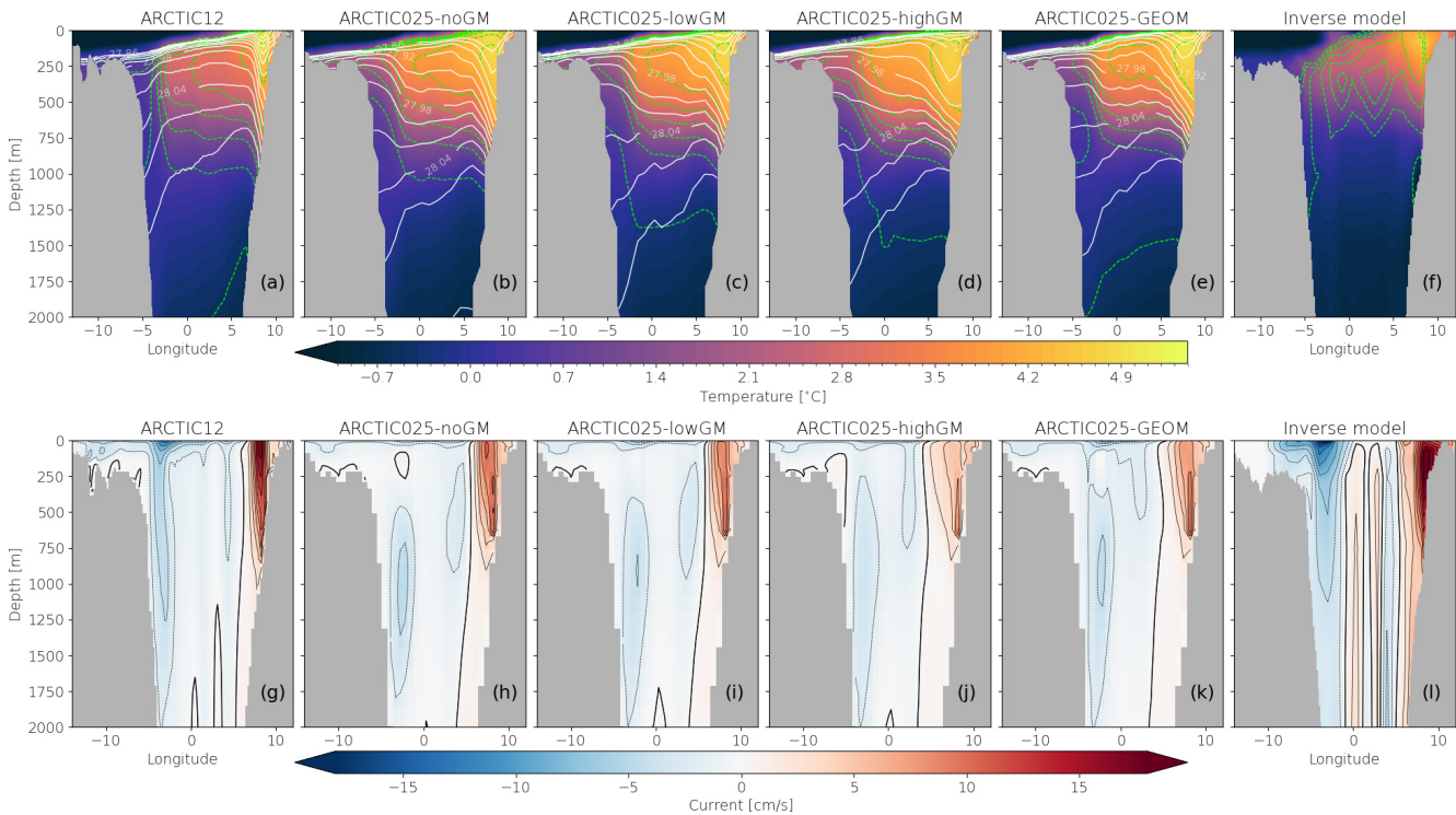
Figure 9. Time-mean (2008–2017) Fram Strait (78° N) potential temperature, density and salinity (a–f), and cross-sectional current (g–l) for the different experiments as well as observational estimates based on an inverse model.
