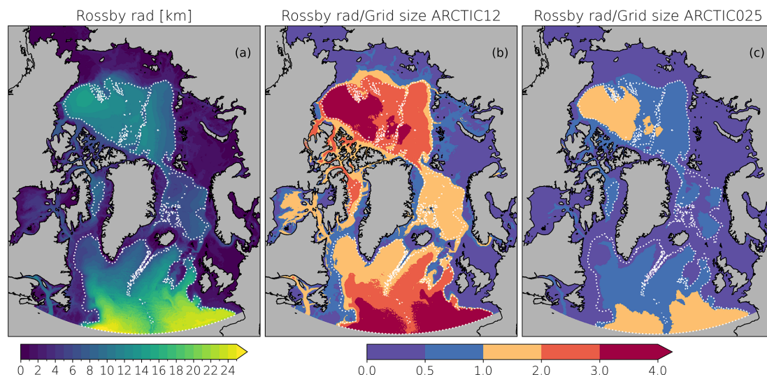
Figure 2. The first baroclinic deformation (Rossby) radius L_d [km] computed from the 1/12^\circ configuration ARCTIC12 (left), the ratio of L_d/\min(dx, dy) for ARCTIC12 (middle) and for the 1/4^\circ configuration ARCTIC025 (right). At a ratio greater than 1.0 the model configurations has at least two grid points per L_d and starts to resolve most of the eddy field. All fields are averaged over the period 1979–2017. The white dotted line shows the 1500 m depth contour.
