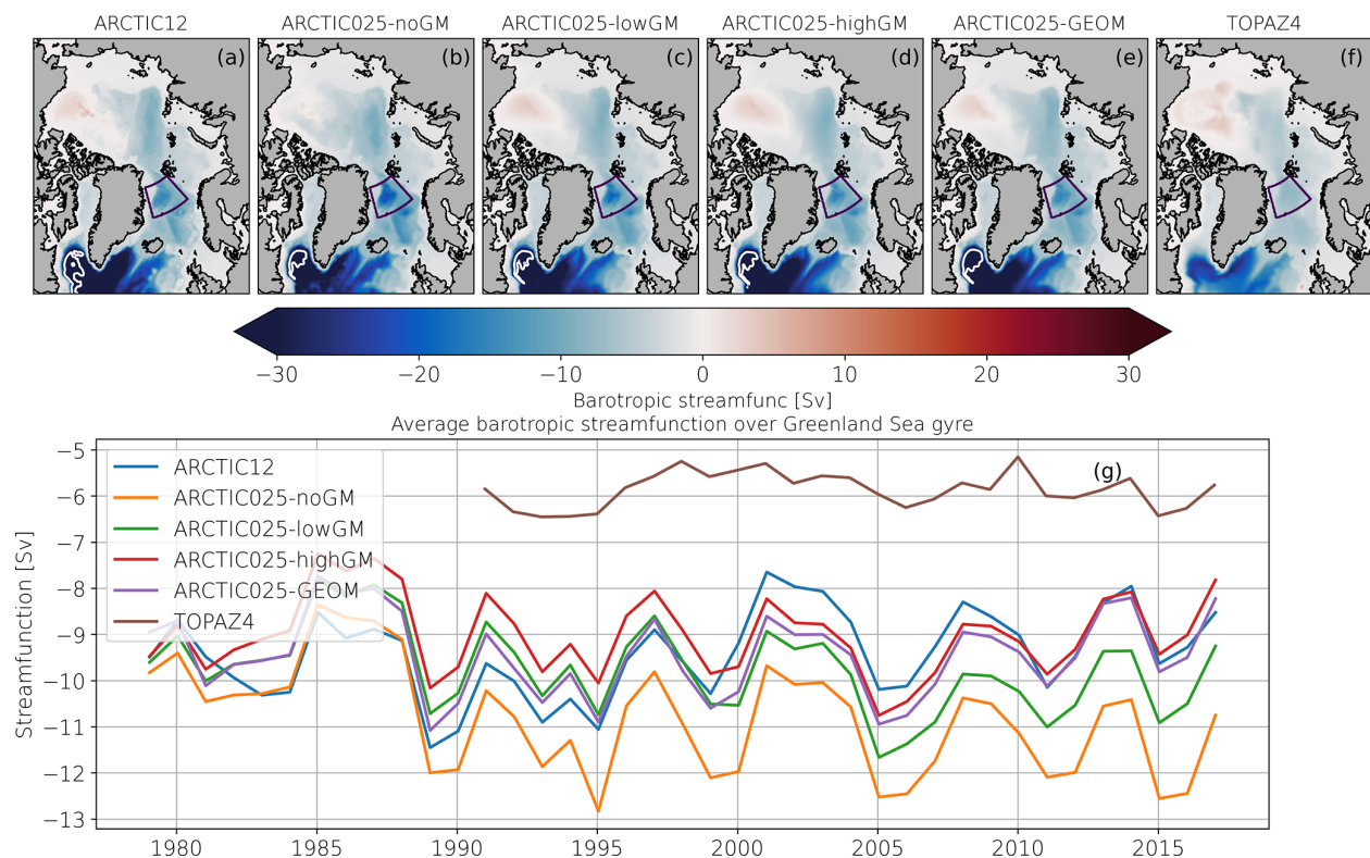
Figure 5. Panels (a)–(e) show the time-mean (2008–2017) barotropic streamfunction [Sv] for the ARCTIC12, ARCTIC025-noGM, ARCTIC025-lowGM, ARCTIC025-highGM, and ARCTIC025-GEOM, respectively. Panel (f) shows the barotropic streamfunction for the TOPAZ4 reanalysis averaged over the same period, and (g) show the yearly mean temporal evolution of the spatial averaged barotropic streamfunction. The Greenland Sea Gyre spatial averaging is done over the purple box shown in (a)–(f), and the white lines show the -45 Sv isoline in the subpolar gyre.
