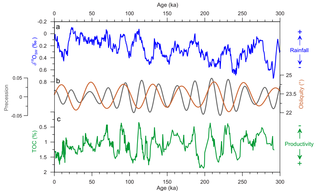
Figure 2. Orbital changes in reconstructed AIM rainfall and wind over the past 300 ka. (a) Seawater \delta^{18}\text{O} of the IPWP records (blue) indicating rainfall-driven changes in ocean salinity [41]. (b) Precession (gray) and obliquity (orange) indices [103]. (c) Total organic carbon (TOC, green, inverted axis) content in marine sediments offshore southwest Sumatra, indicating AIM wind-related changes in upwelling intensity [43]. For locations, see cyan dots in Fig. 1. For spectral power, the reader is referred to the original publications.
