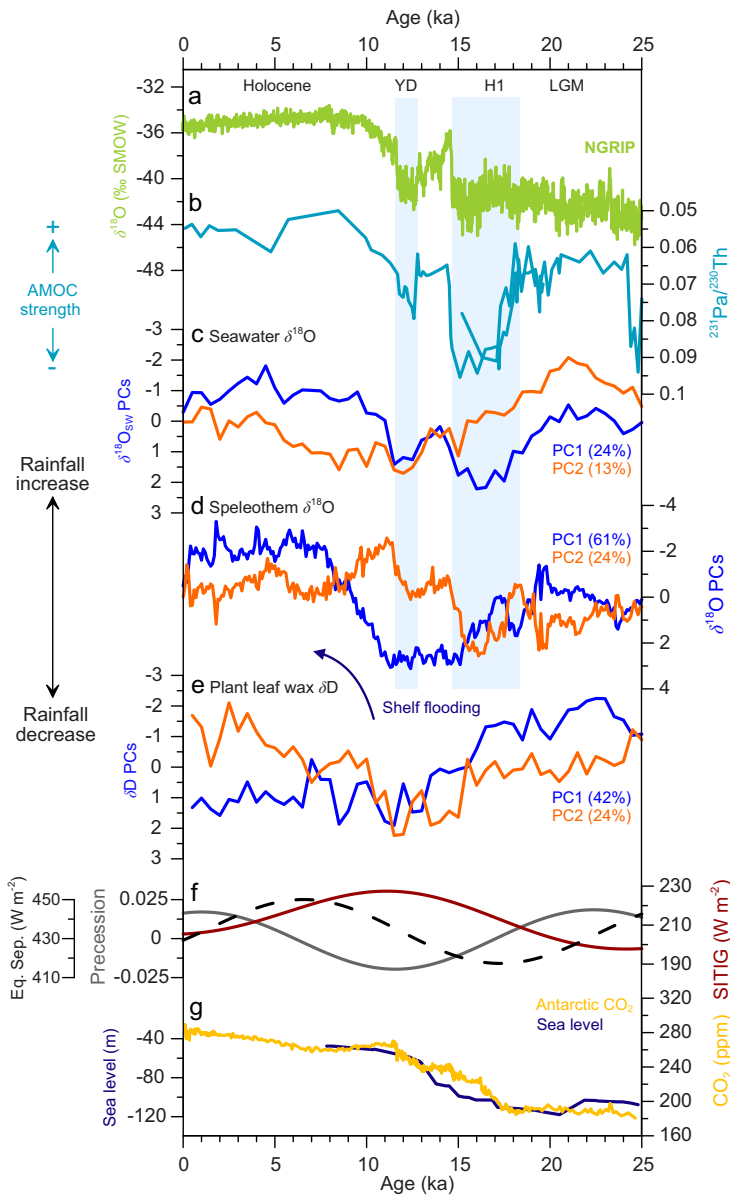
Figure 3. Millennial changes in isotope-based AIM proxy records. (a) \delta^{18}\text{O} data of Greenland ice core NGRIP [104,105] in per mil (‰) standard mean ocean water (SMOW). (b) ^{231}\text{Pa}/^{230}\text{Th} records from the Bermuda Rise [106,107] as indicator for the strength of the AMOC. (c, d and e) 1st (blue) and 2nd (orange) principal components (PCs) of seawater \delta^{18}\text{O} (c), speleothem \delta^{18}\text{O} (d), and plant leaf wax \delta\text{D} (e) records. For site locations, see Fig. 1. (f) Precession index (gray), equatorial September insolation (dashed black) [103], and SITIG [46] (red, 21 June insolation 23^\circ\text{N} – 21^\circ\text{S} ) in Watt per square meter ( \text{W m}^{-2} ). (g) Antarctic composite ice core \text{CO}_2 (yellow) [108] in part per million (ppm), and regional sea level (blue) [109] in meters (m) relative to today. Vertical blue bars indicate Heinrich Stadial 1 (H1) and the Younger Dryas (YD). LGM, Last Glacial Maximum.
