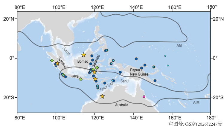
Figure 1. Location of the AIM proxy records. Map of the locations of seawater \delta^{18}\text{O} (blue and cyan dots) and \delta\text{D} records (green diamonds) from lakes and marine sediments, and \delta^{18}\text{O} records of cave speleothems (yellow stars) shown in Fig. 3. Marine records indicated by cyan color are additionally shown in Fig. 2. The magenta dot denotes the location of Lynch's Crater deposits. The thick gray lines indicate the boundaries of the AIM and the Asian monsoons (AM) according to ref. 102, light blue–white areas show the continental shelf regions. For references and sources, see Table S1.
