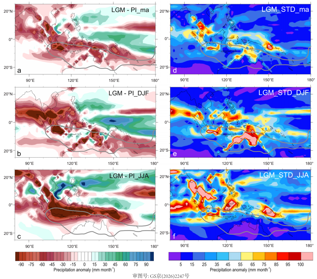
Figure 5. Ensemble mean precipitation anomalies (mm month -1 ) for the LGM relative to pre-industrial. (a–c) and (d–f) same as Fig. 4 but for the LGM using the three PMIP4-CMIP6 models INM-CM4-8, MPI-ESM1-2-LR, and AWI-ESM-1-1-LR. Model outputs for all simulations were downloaded from the Earth System Grid Federation (ESGF; https://esgf-node.llnl.gov/ ).
