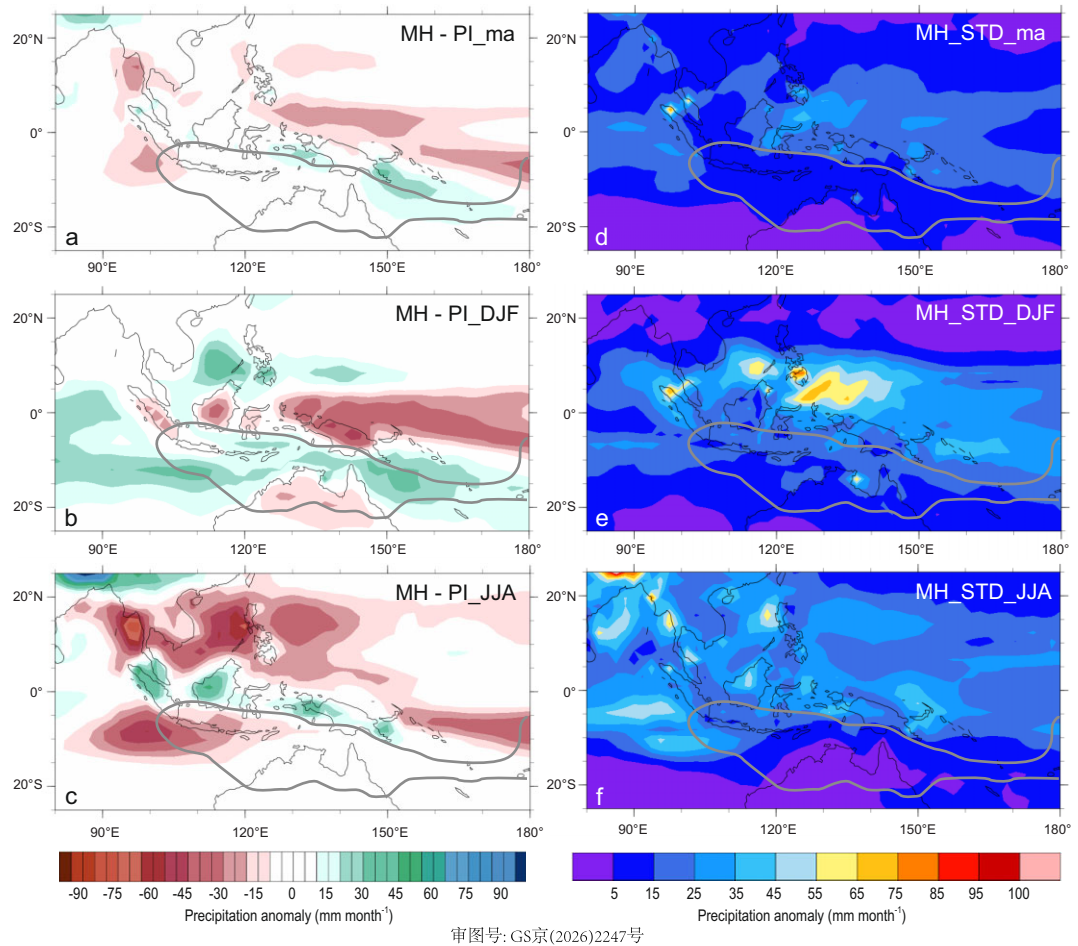
Figure 4. Ensemble mean precipitation anomalies (mm month -1 ) for the mid-Holocene relative to pre-industrial. (a–c) Simulated mid-Holocene (MH) minus pre-industrial (PI) precipitation in mm month -1 for (a) mean annual (ma), (b) the rainy season from December to February (DJF), and (c) the windy season from June to August (JJA). (d–f) Inter-model spread of the mid-Holocene climate response, expressed as the ensemble standard deviation of the 100-year mean MH-PI differences across the 10 PMIP4-CMIP6 models. The ensemble mean is based on 10 PMIP4-CMIP6 models (ACCESS-ESM1-5, AWI-ESM-1-1-LR, CESM2, EC-Earth3-LR, GISS-E2-1-G, HadGEM3-GC31-LL, INM-CM4-8, IPSL-CM6A-LR, MPI-ESM1-2-LR, and NorESM2-LM). Ensemble means and differences were averaged over the final 100 years of the simulations. Thick gray lines indicate the modern boundary of the AIM. Model outputs for all simulations were downloaded from the Earth System Grid Federation (ESGF; https://esgf-node.lnl.gov/ ).
