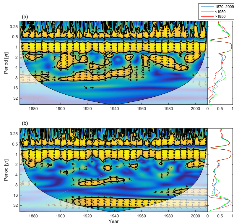
Figure 15. Wavelet coherence between mixed-layer salinity and phosphate concentration (a) and mixed-layer salinity and DIN (b) . Arrows pointing downwards indicate salinity preceding mixed-layer phosphate / DIN by 90°, while arrows pointing upwards mean mixed-layer phosphate / DIN preceding salinity by the same amount. The right panels show the coherence averaged over the whole period (blue) and before (green) and after (red) 1950.
