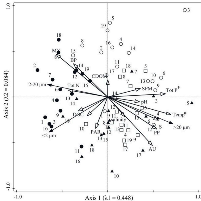
Fig. 5. Redundancy analysis (RDA) ordination plot of the relative contribution of phytoplankton size-structure: pico- (< 2 µm), nano- (2–20 µm), micro- (> 20 µm) phytoplankton, and physicochemical (DOC, CDOM, Tot P, Tot N, Temp, PAR at 1m, SPM, salinity, pH) and biological (primary production (PP), bacterial production (BP), the relative biomass of autotrophs and mixotrophs (AU, MX), taxonomic richness (S)) variables during the study period (● – May; ○ – June, □ – July, ▲ – August). Asterisks indicate statistical significance ( p < 0.05 ) of physicochemical variables influencing the relative contribution of phytoplankton size-structure based on RDA, forward selection method.
