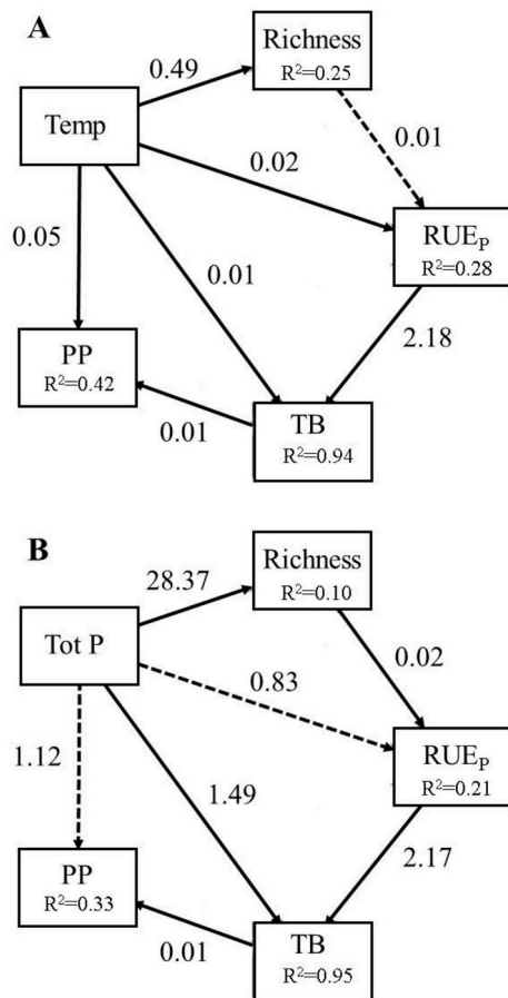
Fig. 7. Path diagram for structural equation model relating temperature, Temp (A), and total phosphorus, Tot P (B), to taxonomic richness, resource use efficiency (RUEp), total phytoplankton biomass (TB) and primary production (PP). The numbers next to each arrow are unstandardized regression coefficients of the SEM. Solid black arrows represent significant paths ( p < 0.05 ) while dash arrows non-significant paths ( p > 0.05 ).
