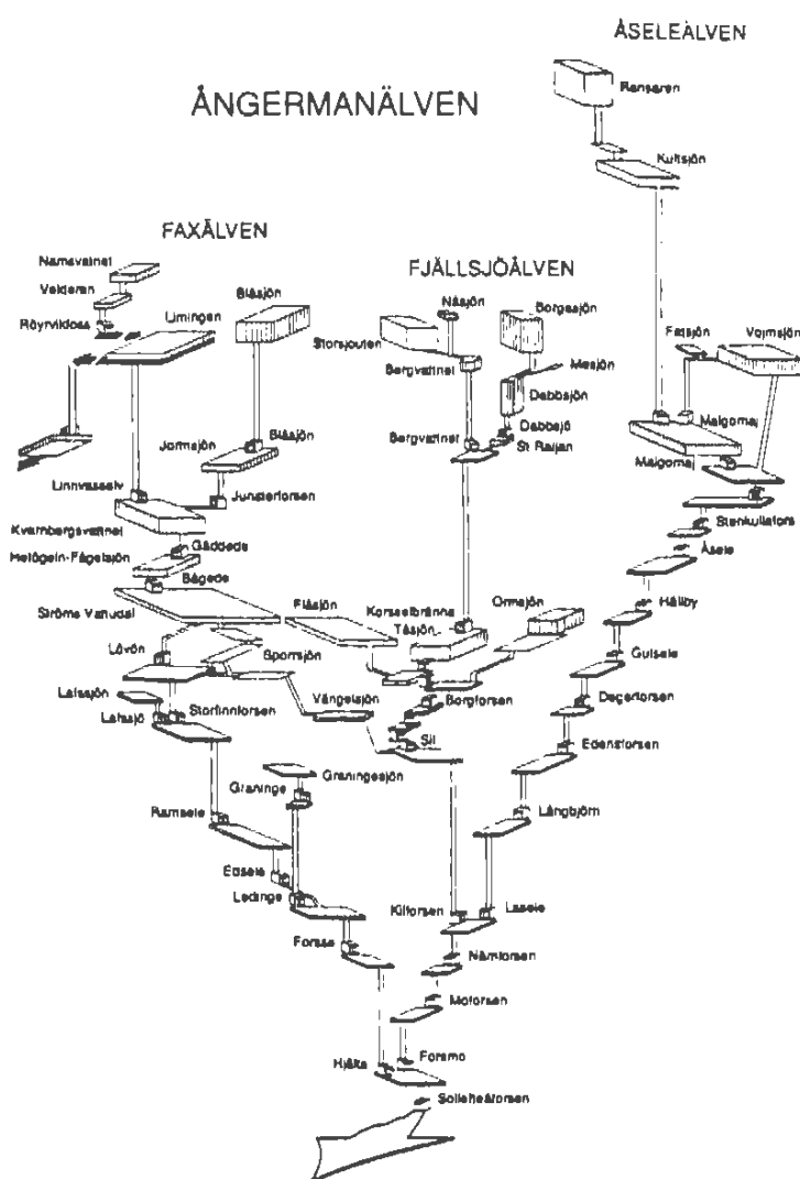
Figure 3.1. Schematic sketch of the hydropower system in the highly regulated river Ångermanälven and its tributaries.
