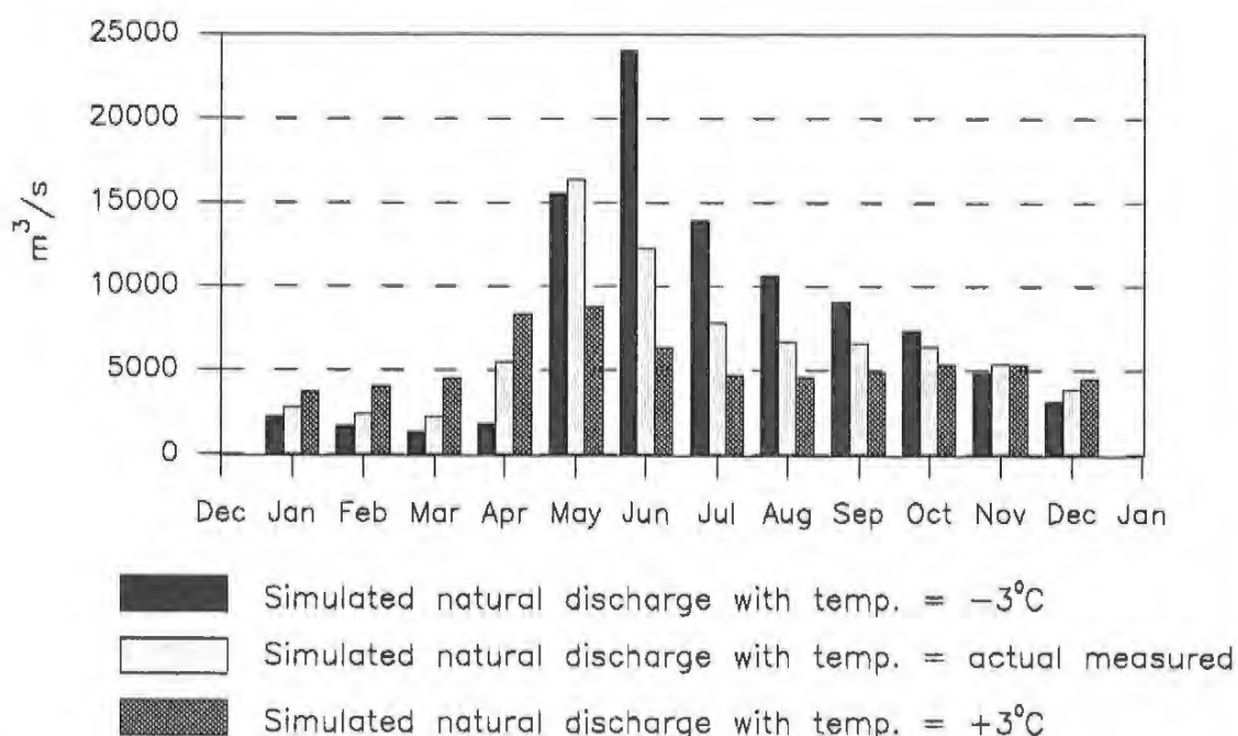
Figure 7.11. Simulated natural discharge at three different temperatures from Sweden and Finland to the Gulf of Bothnia. Monthly means 1981-91.
