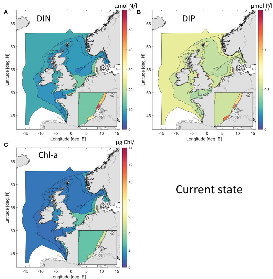
FIGURE 7 Weighted ensemble results for the current state (2009–2014 average), for surface DIN (A), DIP (B) and Chl (C).
