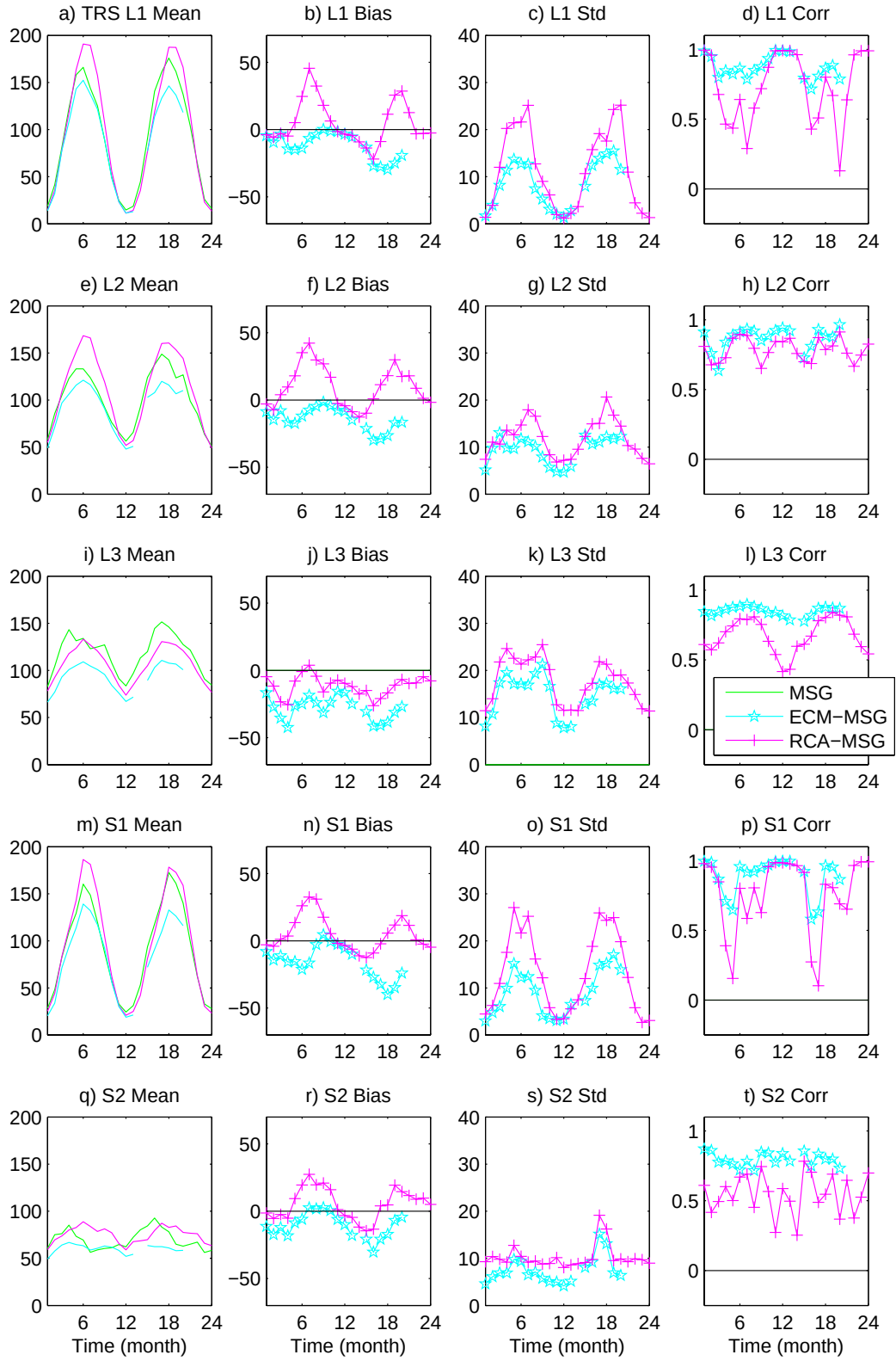
Figure 16. The TOA reflected solar radiation (W/m 2 ), same variables and regions as in Figure13.
