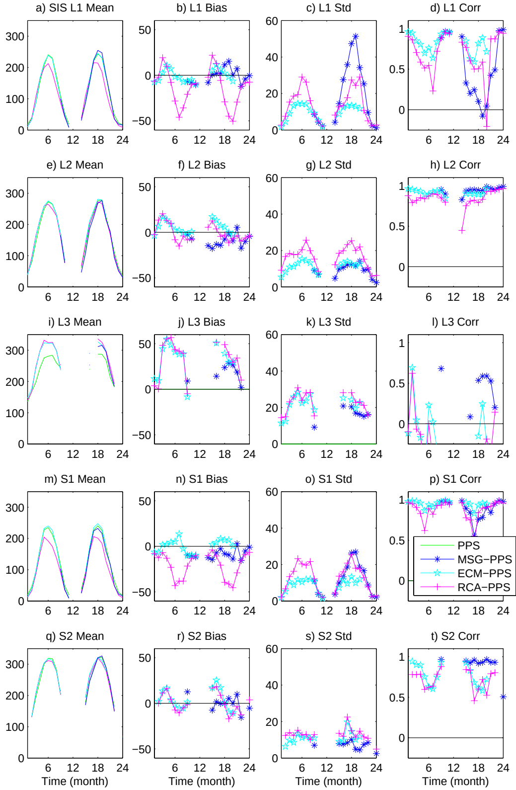
Figure 18. The surface incoming solar radiation (W/m 2 ), same variables and regions as in Figure13.
