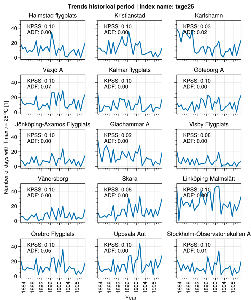
Figure A3. Trend analysis of the historical period (1882–1911) for the txge25 index. KPSS \leq 0.05 indicates that a series is non-stationary. ADF \leq 0.05 indicates that a series is trend stationary.
