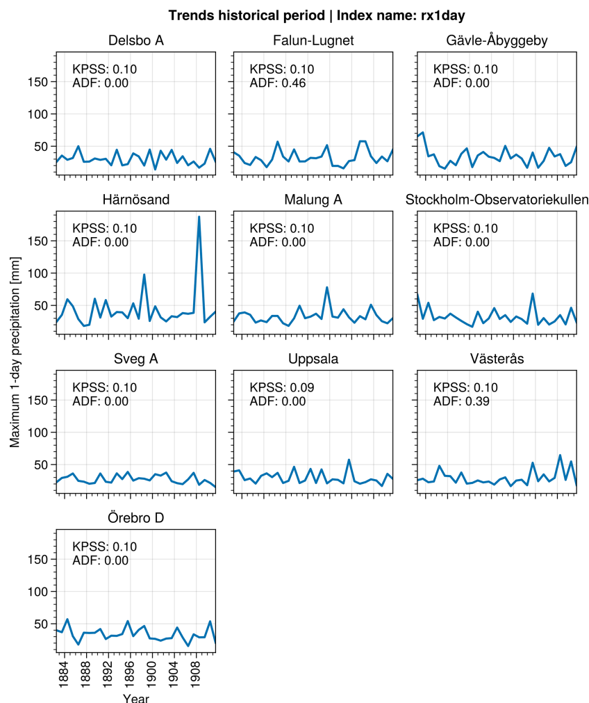
Figure A5. Trend analysis of the historical period (1882–1911) for the Rx1day index. KPSS \leq 0.05 indicates that a series is non-stationary. ADF \leq 0.05 indicates that a series is trend stationary.
