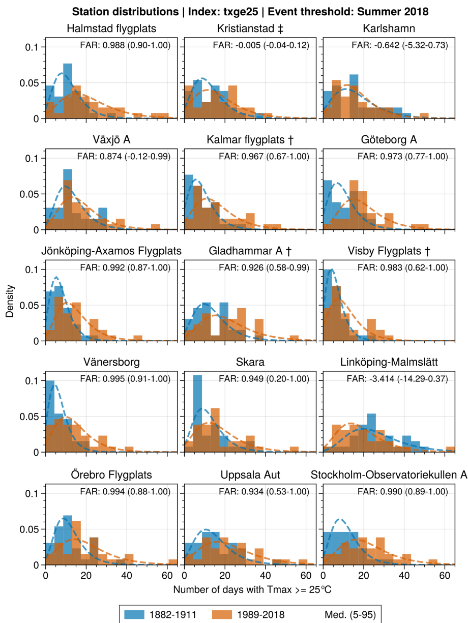
Figure 3. Histograms of the txge25 index for the periods 1882–1911 and 1989–2018. Dashed lines show the probability density function (PDF) of the Gumbel distribution fit to each period. † indicates that at least 1 year misses 15 % of the days in the pre-industrial period. ‡ is the equivalent for the current period.
