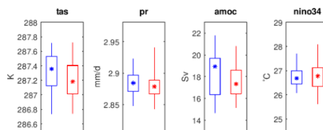
Figure 1. Ensemble spread in the first year after the initialization of the large ensemble (red), compared to the ensemble spread of the regular EC-Earth3 ensemble for the year 1970 of the historical experiment for CMIP6 (blue). The whiskers denote the full ensemble spread (min–max), the boxes the 25th to 75th percentile range, and the stars the median of the distribution. Tas and pr are the annual global mean near-surface temperature and precipitation, respectively. AMOC is the annual average of the monthly maximum Atlantic Meridional Overturning Circulation at 26.5^\circ N. Nino34 is the annual average sea surface temperature (SST) in the Nino3.4 region ( 5^\circ N– 5^\circ S, 170 – 120^\circ W).
