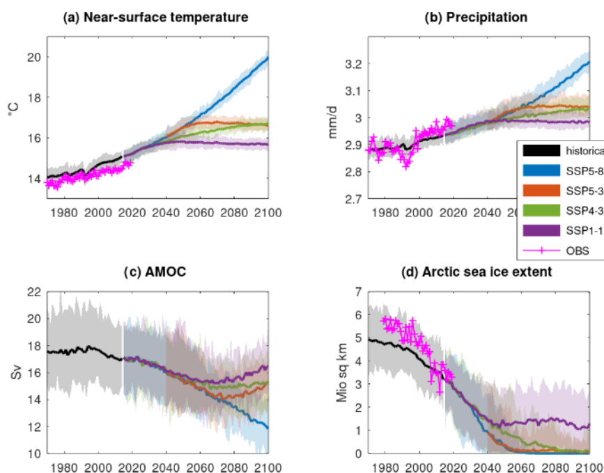
Figure 2. Time series of global annual mean near-surface temperature, precipitation, AMOC, and minimum Arctic sea ice extent in the historical and scenario experiments. Thick lines denote the ensemble means and shaded area the full ensemble width. The scenarios branch off from the historical experiment in 2015 except for SSP5-3.4-OS, which branches off from SSP5-8.5 in 2040. The magenta lines marked with plus signs denote ERA5 (Hersbach et al., 2020) for temperature and precipitation and the OSI-450 sea ice observations (Lavergne et al., 2019).
