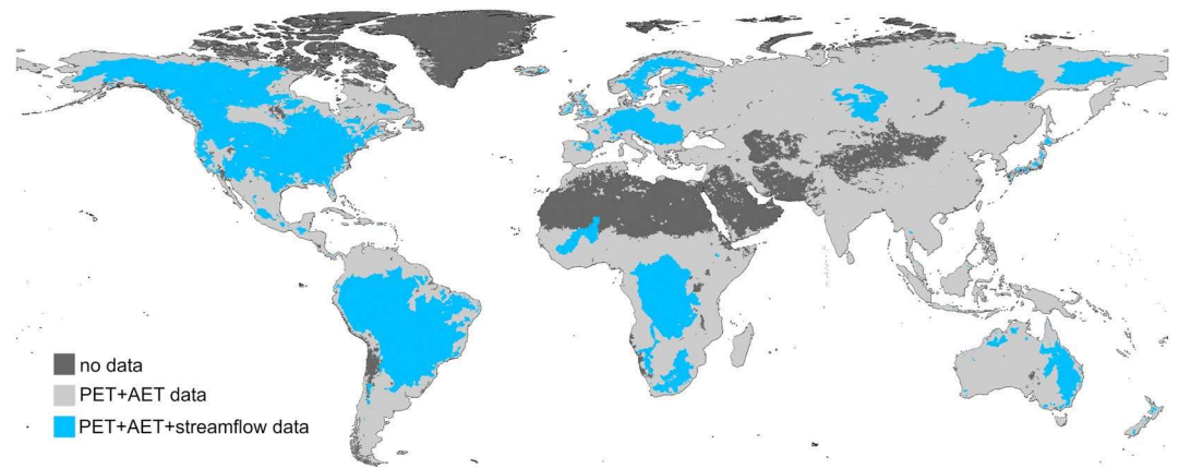
Figure 1. Location of the analyzed catchments: dark gray represents areas without information, light gray represents catchments with information from MODIS (potential evapotranspiration (PET) and actual evapotranspiration (AET)), and light blue represents areas with information from PET, AET and streamflow (upstream areas of the selected streamflow gauge).
