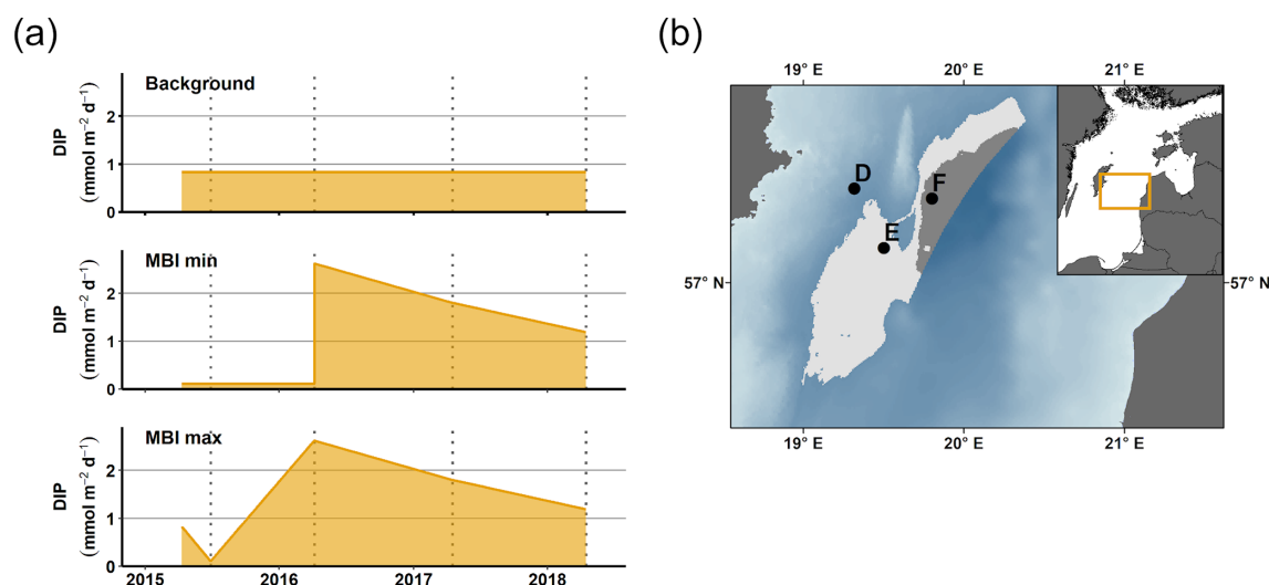
Figure 5. Upscaling of DIP release. (a) DIP release at station F according to three different scenarios: background, MBI min, and MBI max. The lines show the DIP flux according to the different scenarios; the shaded area represents the total DIP release during the period. (b) Sediment areas (western flank of the EGB) used for upscaling calculations. The DIP flux per square metre in the light grey area (150–190 m) is assumed to be the same as at station E, while the dark grey area (> 190 m) is represented by station F. Bathymetric data from the Baltic Sea Bathymetry Database (version 0.9.3); the map was created using the software ArcMap™ (v. 10.6) by Esri.
