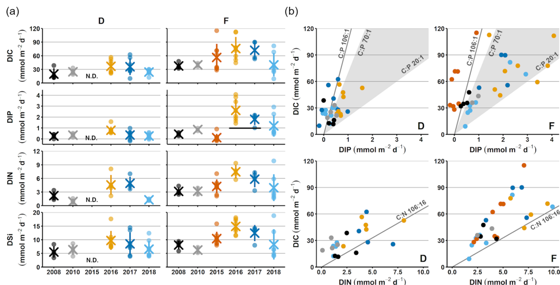
Figure 2. Sediment–water fluxes measured with the benthic chamber lander. Flux data are from before the inflow (2008, 2010; Hall et al., 2017; Nilsson et al., 2019; Viktorsson et al., 2013), right after the inflow (2015; Hall et al., 2017), and post-inflow (2016–2018; this study). (a) Changes in fluxes with time. Small circles mark individual chamber measurements, crosses mark station averages, and lines represent station standard deviations. The black line in the DIP graph for station F in 2016–2017 marks the expected flux for those years, based on the decrease in solid phase inventory. N.D. stands for no data. (b) Fluxes of DIC vs. DIP and DIN. The grey line represents the Redfield ratios of 106 : 1 for DIC : DIP and 106 : 16 for DIC : DIN, the shaded area marks the DIC : DIP ratios between 20 : 1 and 70 : 1. Colour-coding is the same as in (a) .
