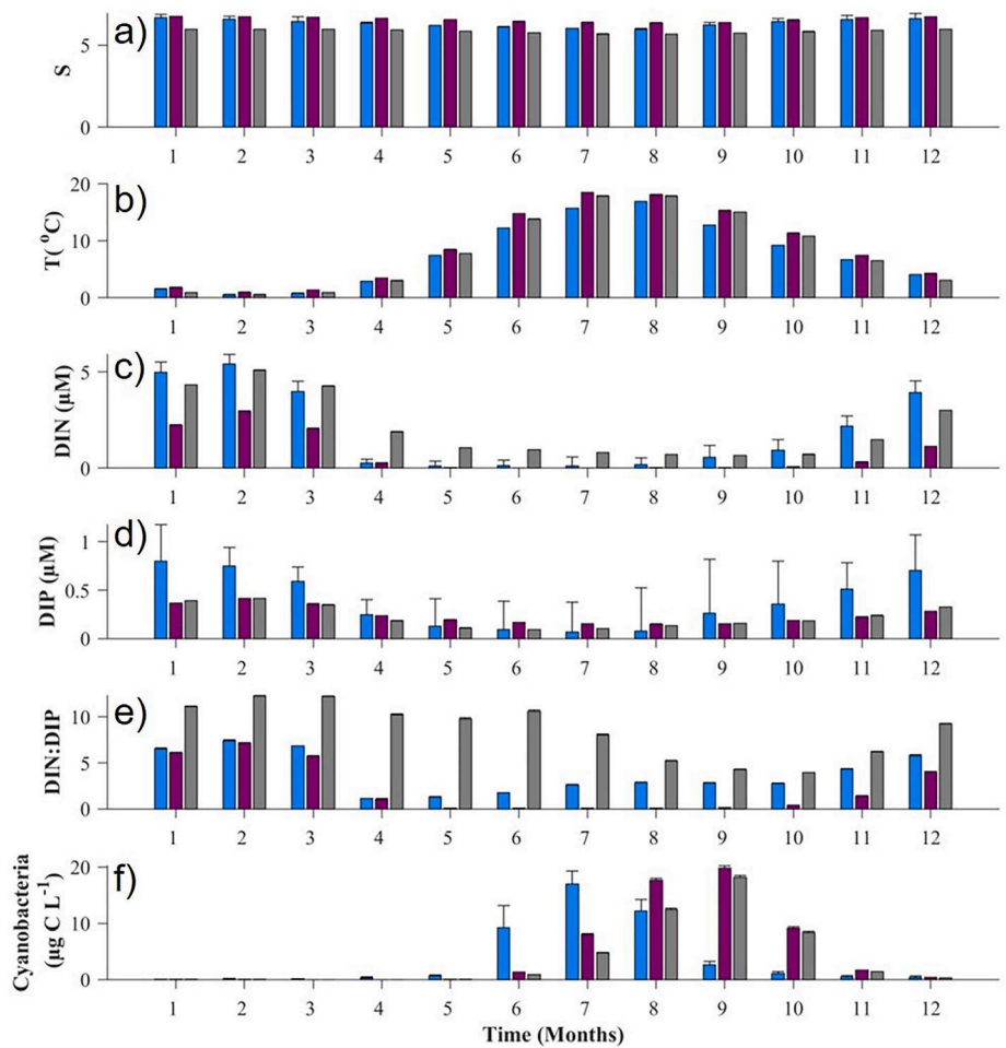
Fig. 2. Seasonal variation of surface (0–10 m), monthly average of a) salinity, b) temperature, c) dissolved inorganic nitrogen (DIN), d) phosphorus (DIP) ratio and f) cyanobacterial carbon biomass of observations (blue) and model (purple) results at the station B1 and for the entire Stockholm archipelago (grey) during the control period 1999–2012. Error bars indicate standard error. Note: error bars for the model are too small to be visible. (For interpretation of the references to color in this figure legend, the reader is referred to the Web version of this article.)
