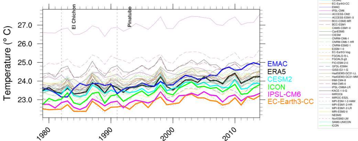
Figure 8. Example of an analysis of native model output alongside CMIP data and reanalysis products with ESMValTool's wide range of diagnostics, similar to Fig. 1 of Bock et al. (2020). Annual near-surface air temperature between 1979 and 2014 averaged over tropical land region (30° S–30° N) for an ensemble of (CMORized) CMIP6 models (thin lines), the ERA5 reanalysis (thick black line), and the models presented in this paper for which a CMOR-like reformatting is available (CESM2: thick cyan line; EMAC: thick blue line; ICON: thick green line; IPSL-CM6: thick magenta line; EC-Earth3-CC: thick orange line). Vertical dashed lines show large volcanic eruptions. For all CMIP6 models and the native output of the models CESM2, EC-Earth3-CC, ICON, and IPSL-CM6, results of an AMIP simulation as defined by CMIP6 (Eyring et al., 2016) are used. The EMAC results shown here are based on a free running EMAC simulation following the CCM1-1 protocol that also uses prescribed sea surface temperatures and sea ice concentrations but a different set of forcings (Jöckel et al., 2016). Due to different model setups, a fair comparison of the individual models is not possible.
