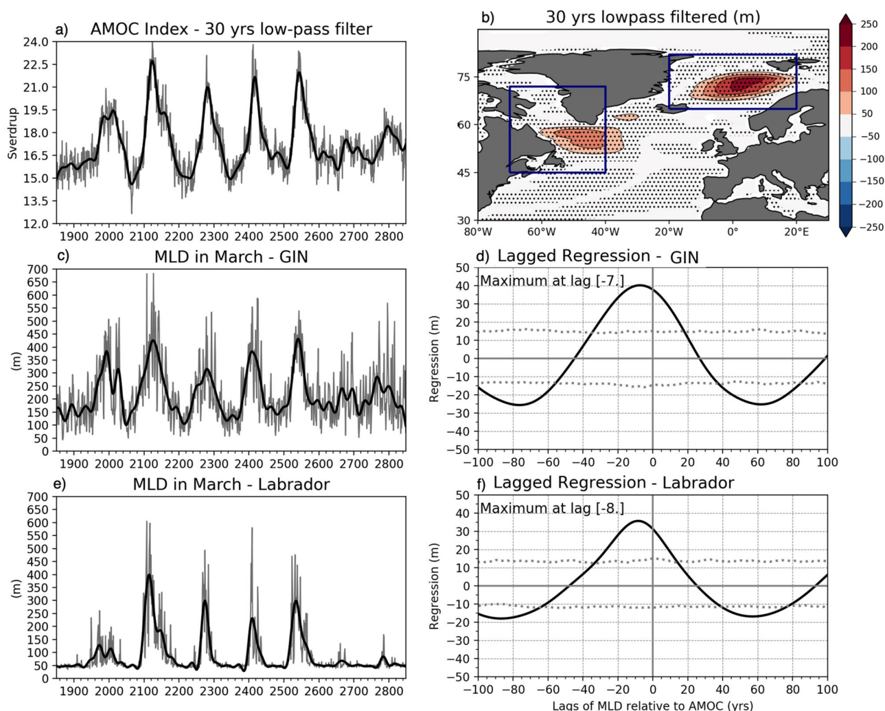
Fig. 3 a Time-series of AMOC index. b Low-frequency MLD (m) in March in the North Atlantic regressed on the AMOC index. c , e Time-series of the mean MLD in March in the GIN and Labrador seas, respectively. d , f Lagged regressions between the AMOC index and the MLD in March in the GIN and Labrador seas. Positive lags
