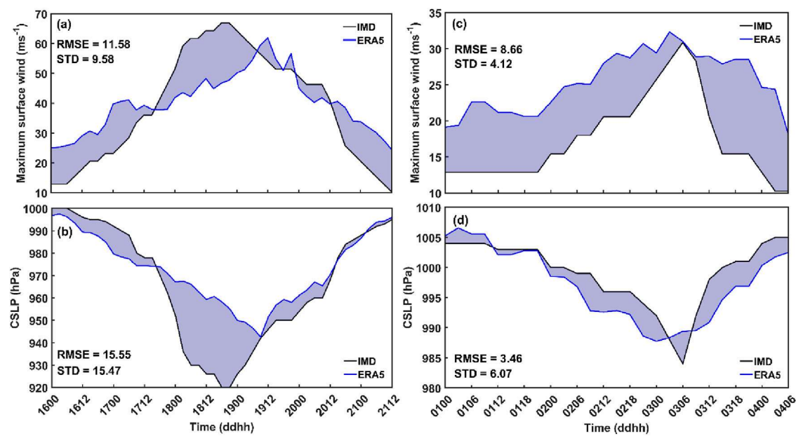
FIGURE 2 Time series of (A, C) maximum sustainable surface wind (MSW; \text{m/sec} ) and (B, D) central sea level pressure (CSLP) in hPa with the comparison of IMD data sets for TC Amphan and Nisarga.
