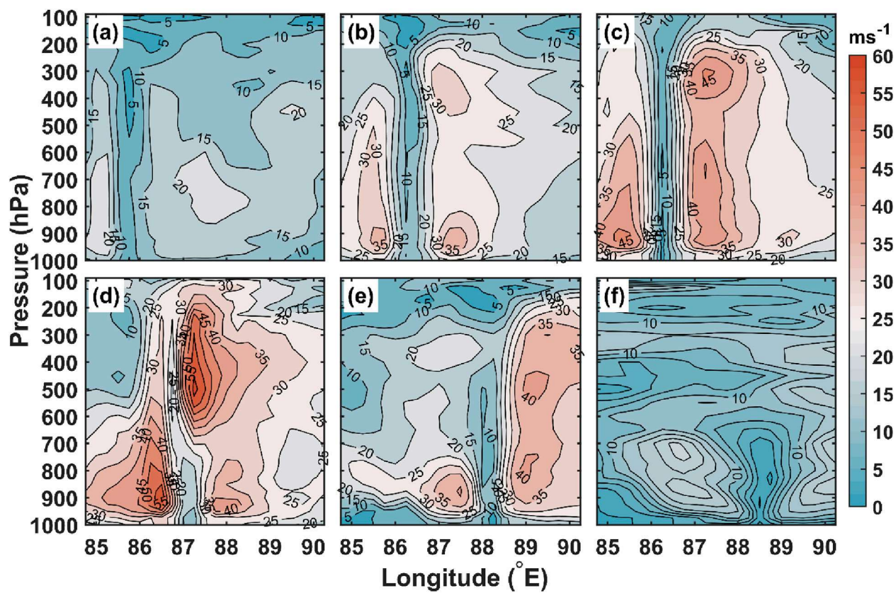
FIGURE 3 East-west cross-section of horizontal wind speed ( \text{m/sec} ) through the center of the cyclone at 12 UTC on (A) 16-May, (B) 17-May, (C) 18-May, (D) 19-May, (E) 20-May, and (F) 21-May for Amphan.
