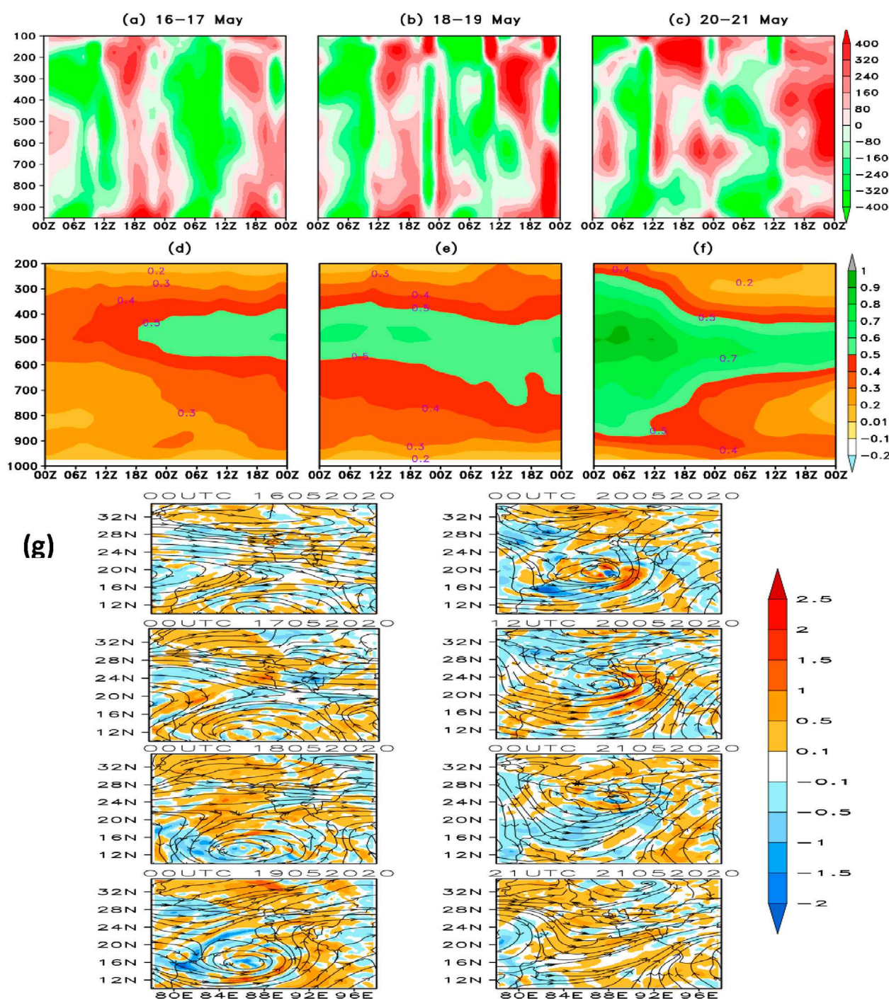
FIGURE 14 Time-pressure cross-section of Diabatic heating ( \text{K sec}^{-1} ) during (A) 00 UTC 16th to 23UTC of 17th May 2020, (B) 00 UTC 18th to 23UTC of 19th May 2020, (C) 00 UTC 20th to 23UTC of 21st May 2020 averaged between 10 and 25° N and 84–94°E from ERA5; (D, E, F) same as (A, B, C) but for potential vorticity ( \times 10^{-6} \text{ K kg}^{-1} \text{ m}^2 \text{ s}^{-1} ); (G) Spatial distribution of vertically averaged (up to 500 hPa) diabatic heating (shaded; \text{K h}^{-1} ) superimposed with 850 hPa streamlines from 00UTC 16th to 21UTC of 21st May 2020.
