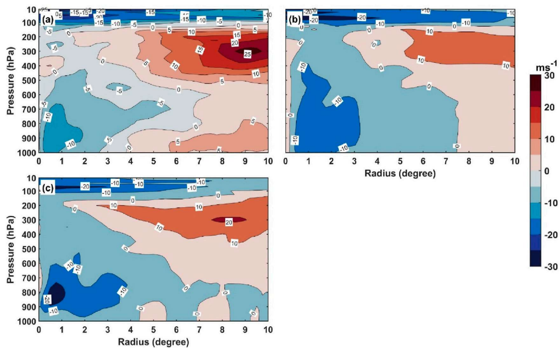
FIGURE 8 Radius (degree)-height (hPa) cross section of radial wind (m/sec) from the TC center at 12 UTC on (A) 01-Jun, (B) 02-Jun, and (C) 03-Jun for Nisarga.
