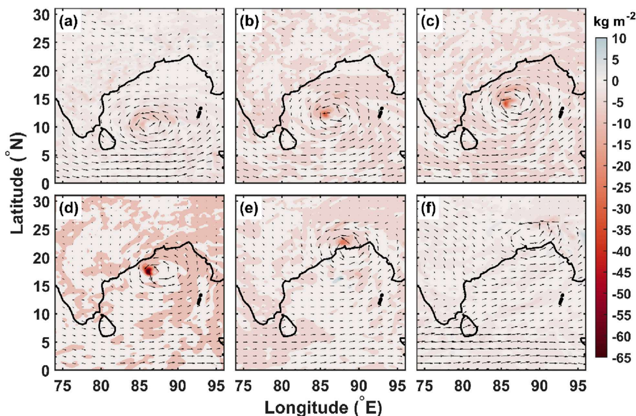
FIGURE 11 The spatial distribution of vertically integrated moisture divergence up to 200 hPa ( \text{kg m}^{-2} , Section 1) at 12 UTC on (A) 16-May, (B) 17-May, (C) 18-May, (D) 19-May, (E) 20-May, and (F) 21-May for TC Amphan.
