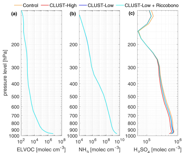
Figure A2. The global mean vertical concentration for modeled gas-phase ELVOCs, \text{NH}_3 , and \text{H}_2\text{SO}_4 . There is negligible model difference for ELVOC as the concentration is steady state, and \text{NH}_3 is not consumed in the NPF function.
