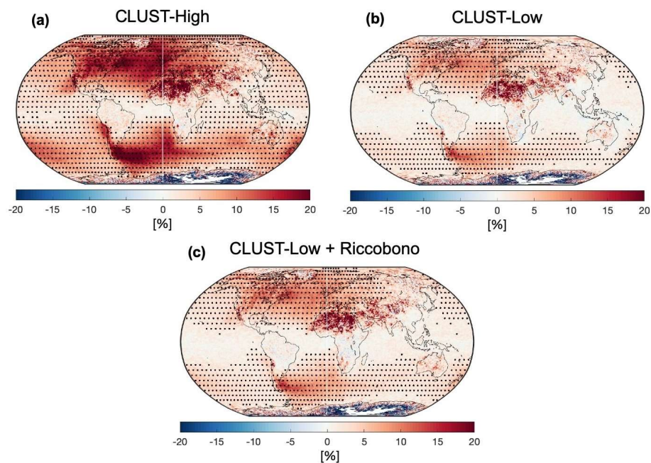
Figure A7. The annual mean difference from the control case of the total column of cloud liquid water ( \text{kg m}^{-2} ), shown as the relative difference, with t -test significance (95 %) shown as dots.
