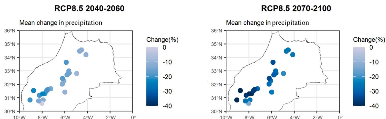
Fig. 6. Spatial Distribution of Mean Relative Change in Precipitation (%) relative to the historical period (1975–2005) for 2040–2060 and 2070–2100.
