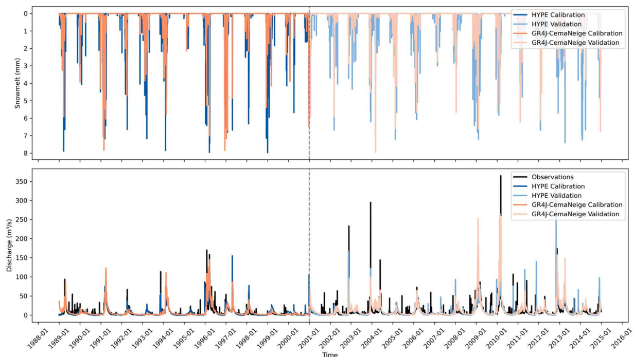
Fig. 3. Representative hydrographs showing observed and simulated daily discharge and snowmelt for a representative basin (Ait Ouchene basin) during calibration and validation periods.
