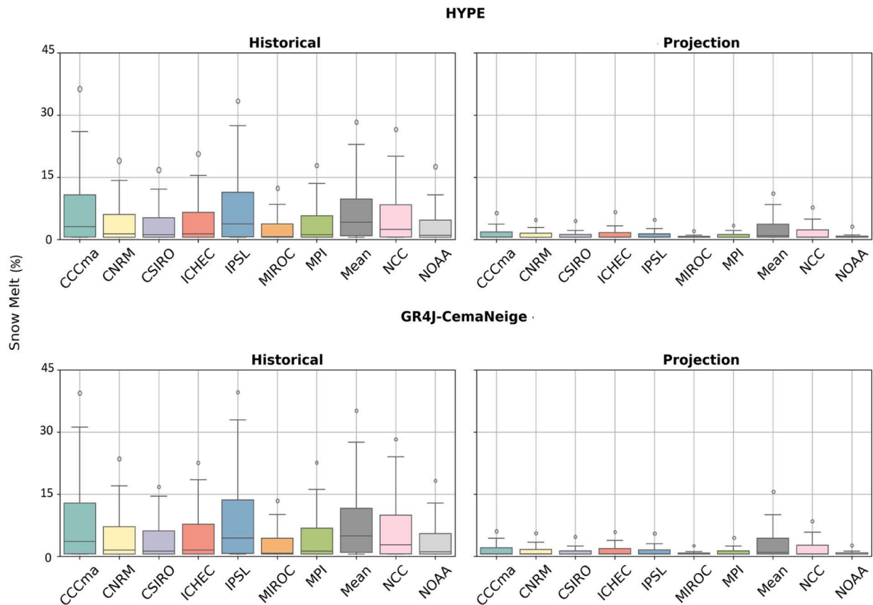
Fig. 12. Boxplots comparing snowmelt Contribution (%) across different climate models for two hydrological models (HYPE and GR4J-CemaNeige) during historical and projected periods.
