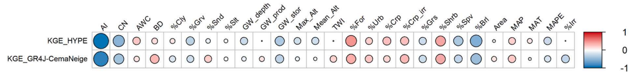
Fig. 5. Correlation Matrix of KGE Scores from HYPE and GR4J-CemaNeige Models and Basin Characteristics., Notes: AI: Aridity Index, CN: Curve Number, AWC: Available Water Capacity, BD: Bulk Density, %Cly: %Clay, %Grv: %Gravel, %Snd: %Sand, %Slt: %Silt, GW_depth: Groundwater Depth, GW_prod: Groundwater Productivity, GW_stor: Groundwater Storage, Max_Alt: Maximum Altitude, Mean_Alt: Mean Altitude, TWI: Topographic Wetness Index, %For: %Forest, %Urb: %Urban, %Crp: %Cropland, %Crp_irr: %Cropland Irrigated, %Grs: %Grassland, %Shrb: %Shrubland, %Spv: %Sparse Vegetation, %Brl: %Bare Land, Area: Basin Area, MAP: Mean Annual Precipitation, MAT: Mean Annual Temperature, MAPE: Mean Annual Potential Evapotranspiration, %Irr: %Irrigation, KGE_HYPE: Kling-Gupta Efficiency of HYPE model, KGE_GR4J-CemaNeige: Kling-Gupta Efficiency of GR4J-CemaNeige model.
