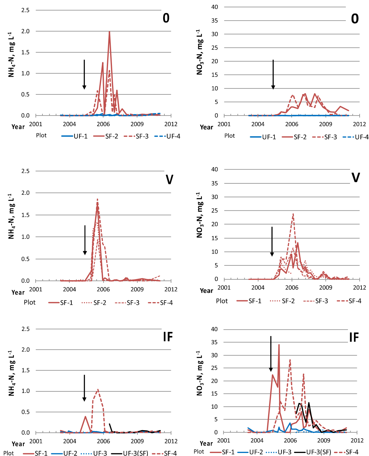
Fig. 3. Concentrations of \text{NH}_4^+\text{-N} (left panel) and \text{NO}_3\text{-N} (right panel) in soil water at 50 cm soil depth in the 0, V, and IF treatments at Skogaby, 2003–2011. Arrows indicate the storm-felling event (January 2005). Storm-felled (SF) plots are indicated by red lines and undisturbed (UF) plots by blue lines, while different numbers (1–4) indicate blocks. For the IF treatment, 'UF-3' indicates the undisturbed part of IF block 3 (2007–2010), while 'UF-3(SF)' indicates the storm-felled part of the same plot and period (black solid line). The sampling in 2004–2006 did not separate storm-felled from undisturbed parts of the plot (data not shown). (For interpretation of the references to colour in this figure legend, the reader is referred to the web version of this article.)
