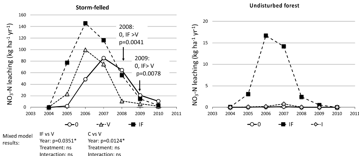
Fig. 4. Mean annual ( n = 2 ) NO 3 -N leaching at 50 cm soil depth in storm-felled 0, V, and IF plots at Skogaby, 2005–2010 (left panel), and corresponding leaching in undisturbed forest plots in the 0, I and IF treatments (right panel). Data from ‘undamaged’ IF block 3 in 2005–2006 are excluded because soil water from the damaged part of the plot was included in analyses, but data from the same plot in 2007–2010 included only samples from the undamaged part. All plots of the I treatment were undisturbed (i.e., n = 4 ). The main storm-felling event occurred in January 2005. Results of mixed model tests and ANOVA by year are shown for p < 0.05 .
