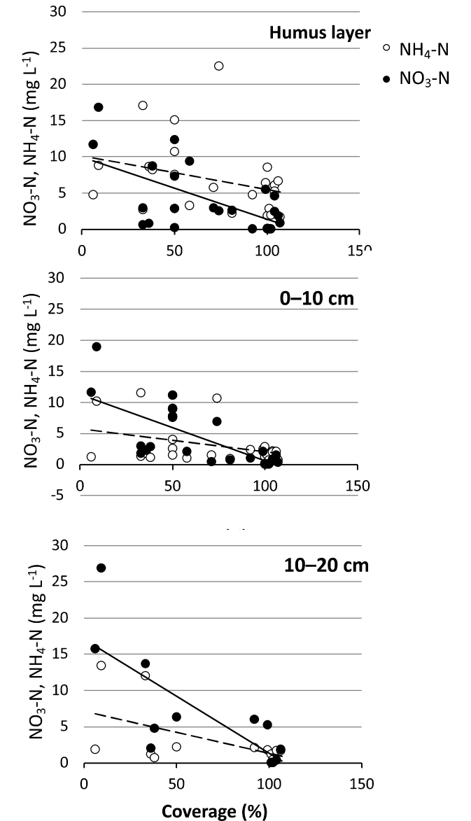
Fig. 7. Soil water concentrations of \text{NH}_4\text{-N} and \text{NO}_3\text{-N} ( \text{mg L}^{-1} ) in different soil horizons in relation to vegetation coverage (%) in July 2008, the third year following storm-felling at Skogaby. The data show spot-scale ( \approx 1 \text{ m}^2 ) correlations between plant coverage and \text{NO}_3\text{-N} (filled symbols, solid regression line) and \text{NH}_4\text{-N} (open symbols, dashed regression line) in soil water, measured in storm-felled 0, V, and IF plots.
