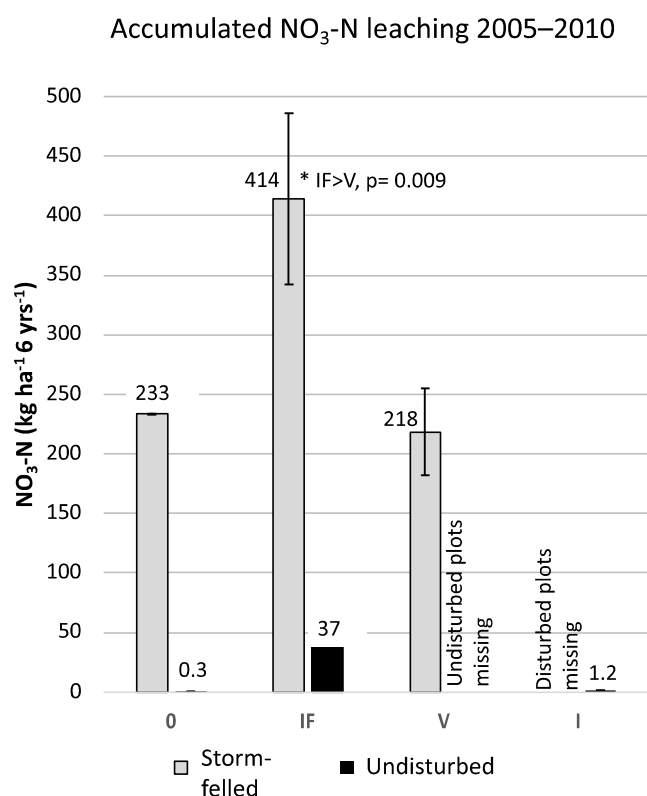
Fig. 5. Treatment means ( \pm SE) of accumulated NO 3 -N leaching (kg ha -1 ) at 50 cm depth during the period 2005–2010. A significant difference between V and IF is indicated (ANOVA). Grey bars = storm-felled stand, black bars = undisturbed stand.
