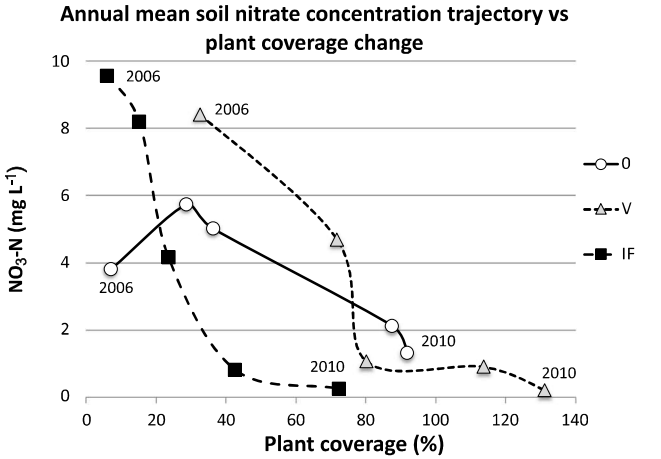
Fig. 8. Change in \text{NO}_3\text{-N} concentrations ( \text{mg L}^{-1} ) in soil water (50 cm) in relation to vegetation coverage (%) during 2006–2010. Means for treatments 0, V, and IF ( n = 2 ), measured at the plot scale. Each line shows the time trajectory going from left (2006) to right (2010). The storm-felling event occurred in January 2005.
