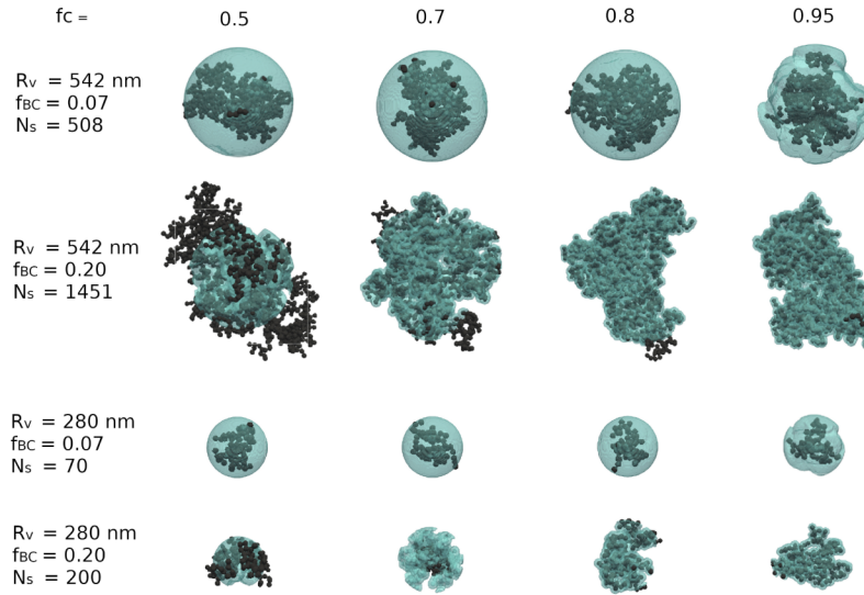
Fig. 1. Reference model of coated BC aggregates. The volume-equivalent sizes are R_v=542\text{nm} (rows 1–2) and 280\text{nm} (rows 3–4), the BC volume fractions are f_{BC}=0.07 (rows 1, 3) and 0.20 (rows 2, 4). The scaling factor f_c of the critical radius in the model in columns 1–4 is 0.5 , 0.7 , 0.8 , and 0.95 , respectively. The figure shows only one out of five stochastic realisations of each model geometry.
