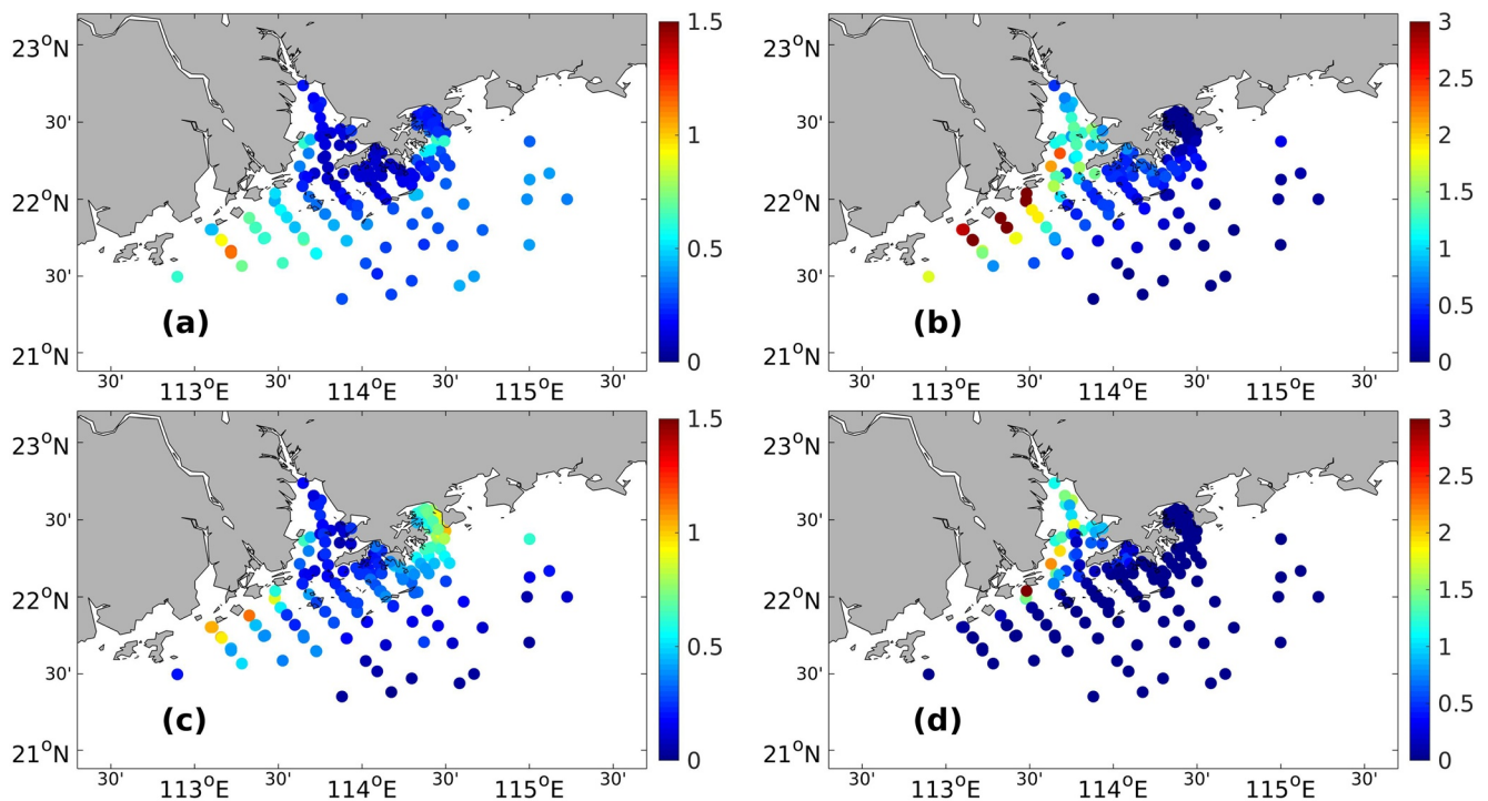
Figure 4. The error variances of the temperature (left panel; unit: (^{\circ}\text{C})^2 ) and salinity (right panel; unit: (\text{g/kg})^2 ) from the snapshot ensemble in DA03 in the surface (a, b) and bottom (c, d) waters at the observation stations.
