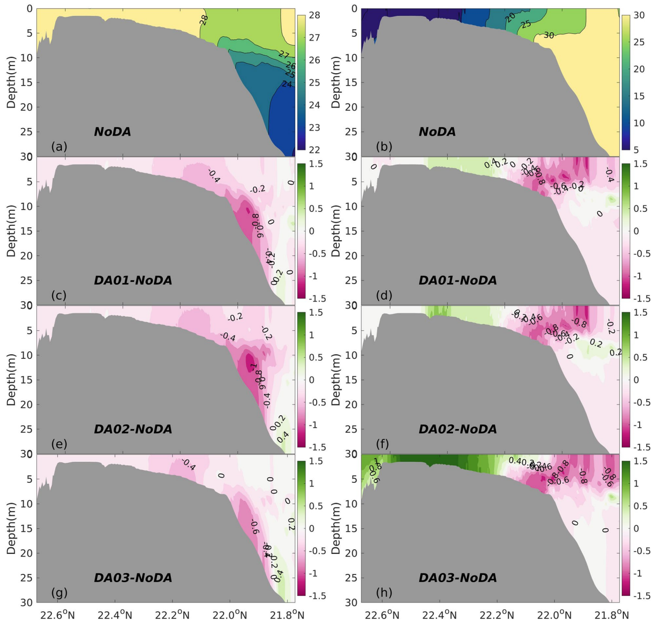
Figure 9. The cross-section (T2, Figure 2a) temperature (left panel; unit: °C) and salinity (right panel; unit: g/kg) simulated by the model, the simulation increment of the assimilation experiments on July 23, 2015.
