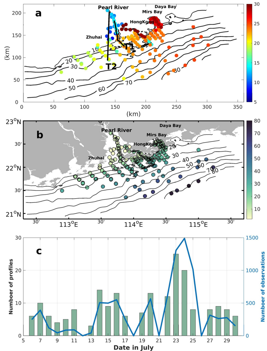
Figure 2. (a) Station locations are color-coded by the date of their occupation and the model domain in Cartesian coordinates. Black lines indicate sections T1 and T2 used in the analysis of Section 4.4; (b) the horizontal coverage and max depth (colorbar) of the observed Conductivity-Temperature-Pressure profiles; (c) the daily number of profiles (bars) and observations (blue line) for temperature (salinity), respectively.
