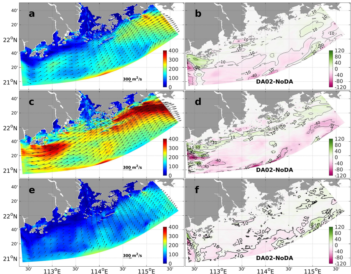
Figure 7. Modeled volume transport per unit depth (left panel; unit: \text{m}^2/\text{s} ) of the control run, the transport difference (right panel; unit: \text{m}^2/\text{s} ) between the DA02 and NoDA for vertical average (a and b), the surface (c and d) and bottom (e and f) at July 25, 2015, respectively. The arrows in the left panel show the direction and magnitude of transport.
