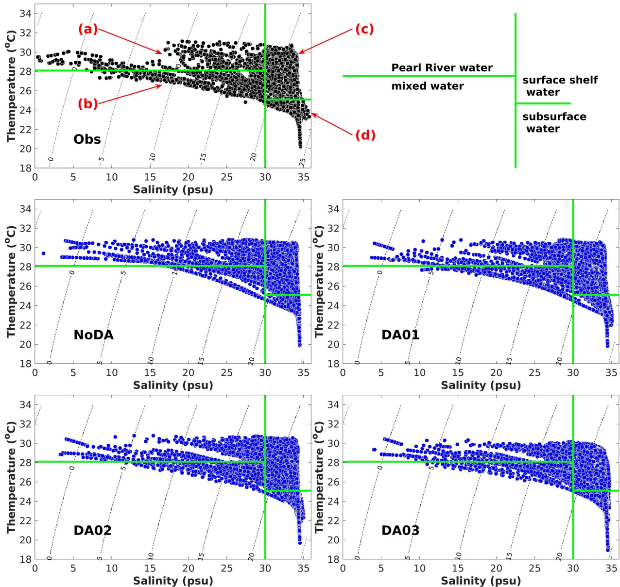
Figure 10. T-S diagram of all sampling stations for observation, NoDA, and data assimilation experiments, respectively. The contour lines denote the sigma-t density (unit: \text{kg/m}^3 ). The arrows show where data assimilation has improved.
