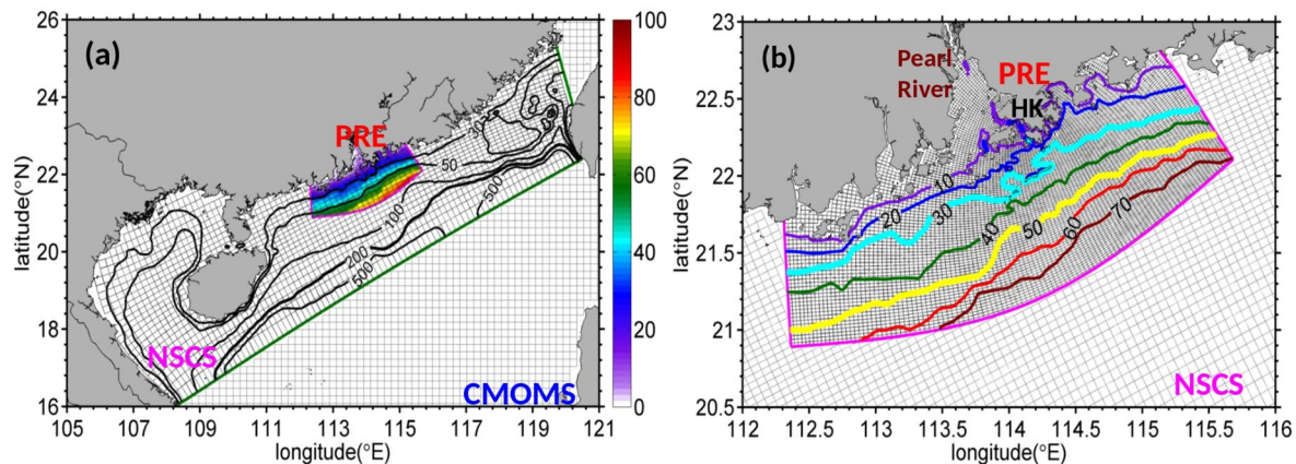
Figure 1. (a) The model domain, bathymetry (unit: m) and the isobaths (color lines) in the Pearl River Estuary and (b) the northern South China Sea (Liu & Gan, 2020) of the China Sea Multi-Scale Ocean Modeling System.
