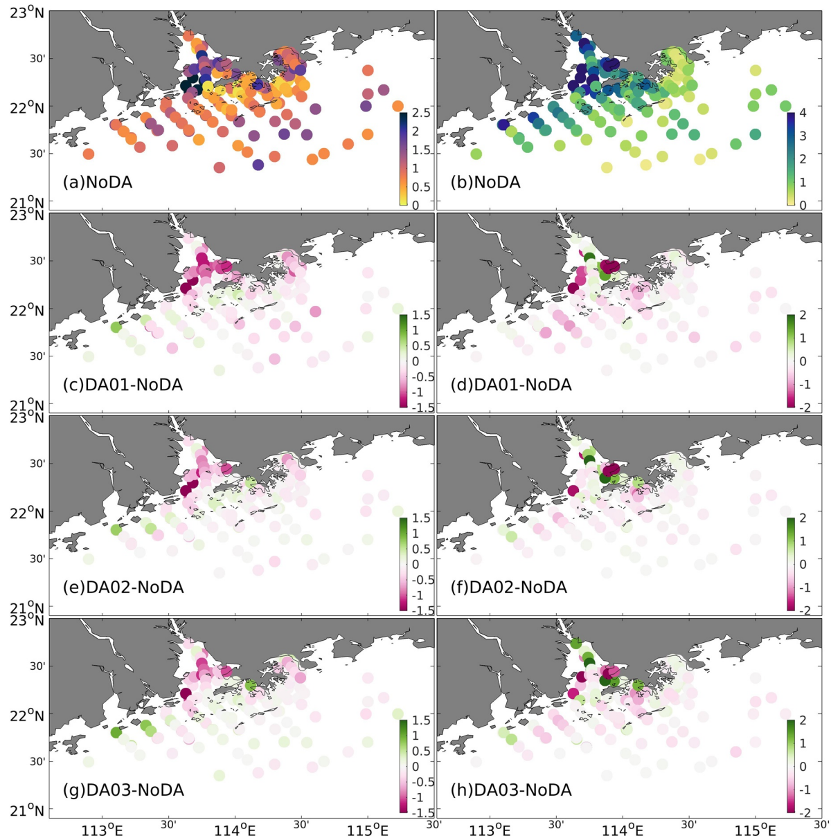
Figure 6. RMSE of temperature (left panel; unit: °C) and salinity (right panel; unit: g/kg) from NoDA relative to the CTD observations in July 2015 and the RMSE adjustments in DA01, DA02, and DA03 relative to NoDA.
