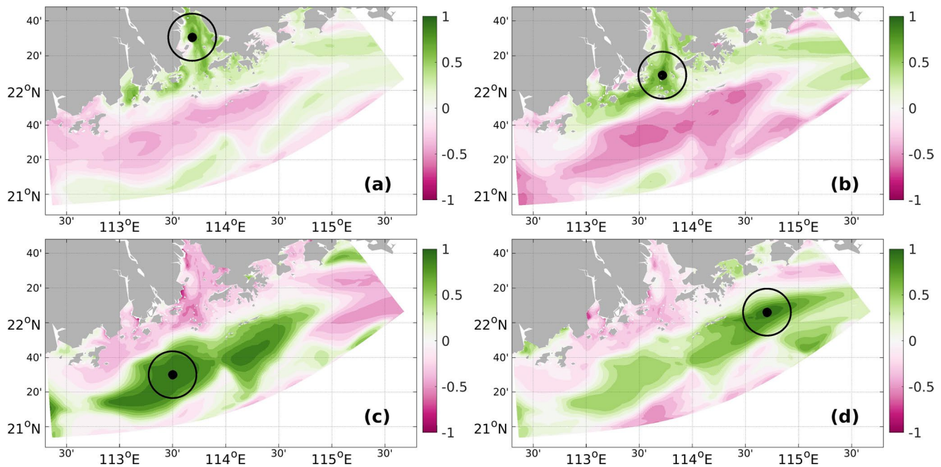
Figure 3. An example of the ensemble-based cross-correlation structure for a temperature observation in the surface cell for (a) Pearl River, (b) Pearl River Estuary, (c) shelf upstream region, and (d) shelf downstream region. Dark dots show the observation position and circles indicate the range of a 20-km influenced radius.
