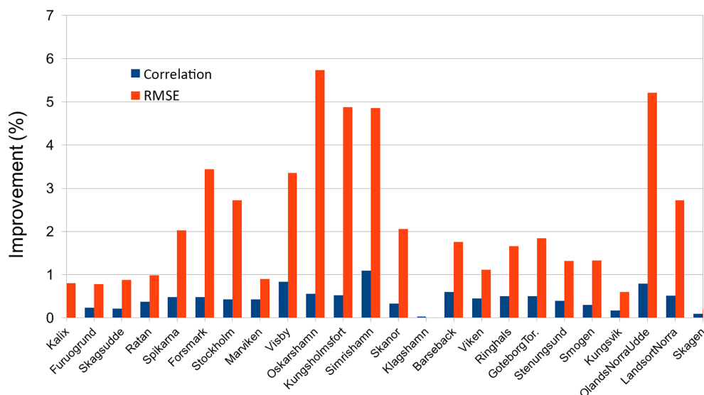
Figure 10. The improvement (%) of correlation and RMSE for the SLA at the tide gauge stations. The station positions are shown in Fig. 8b.
