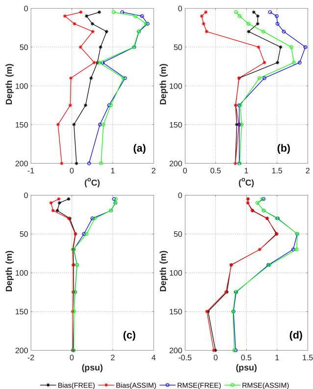
Figure 9. The overall RMSE and bias of temperature (a, b) and salinity (c, d) from FREE and ASSIM relative to observations as a function of water depth inside (b, d) and outside (a, c) of the Baltic Sea.
