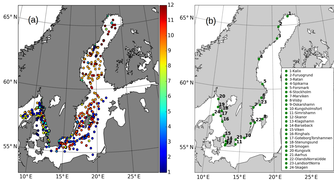
Figure 8. (a) Map of the temperature and salinity profiles from the SHARK database in 2010. The colors show the observation months. (b) The tide gauge stations along the Swedish coast.
