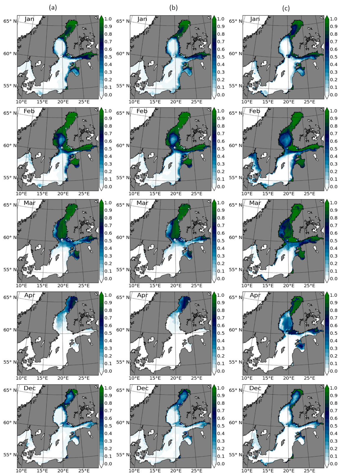
Figure 12. The monthly mean sea-ice concentrations in FREE (a), ASSIM (b) and IceMap (c), respectively.
