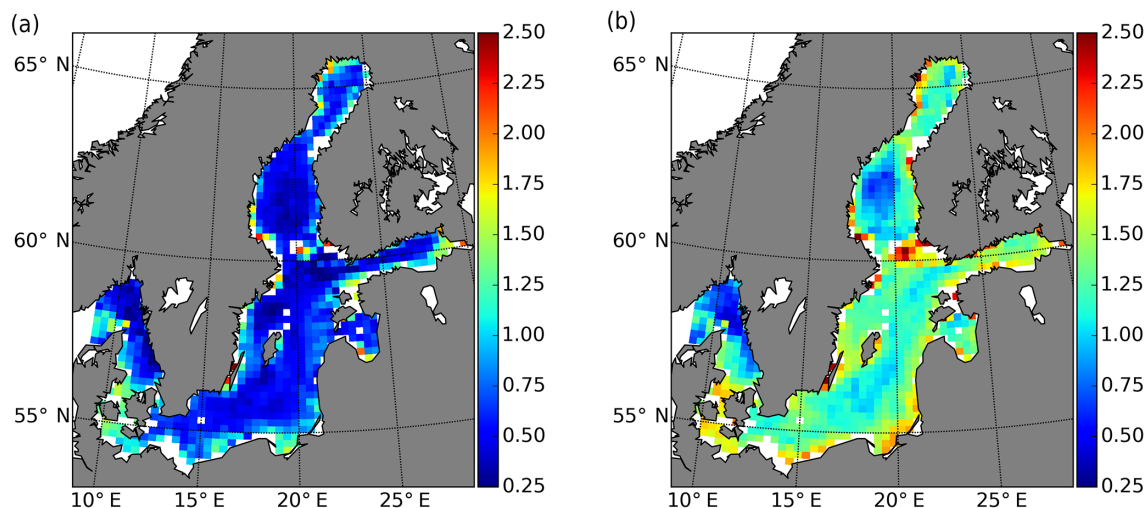
Figure 3. Map of the RMSE of SST from ASSIM (a) and FREE (b) calculated against IceMap SST in 2010, respectively.
