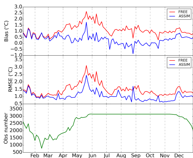
Figure 4. The evolution of basin-averaged bias and RMSE of SST from FREE and ASSIM relative to IceMap SST and the number of IceMap observations in 2010.
