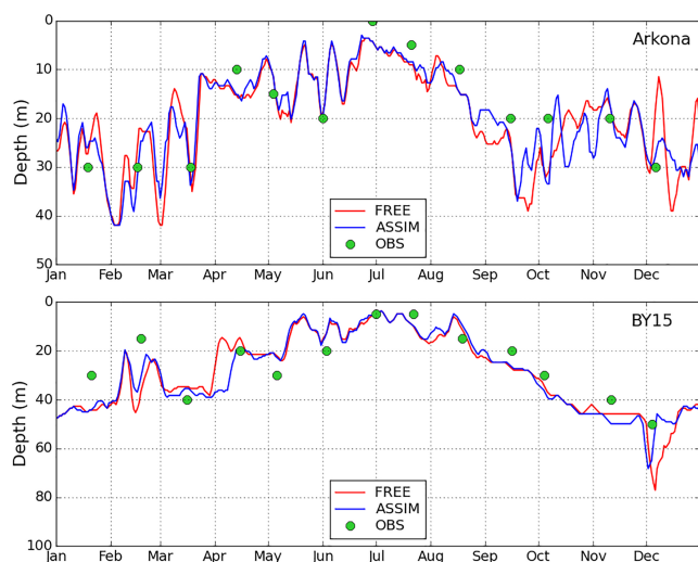
Figure 7. The time series of mixed layer depth at the Arkona and BY15 stations.
