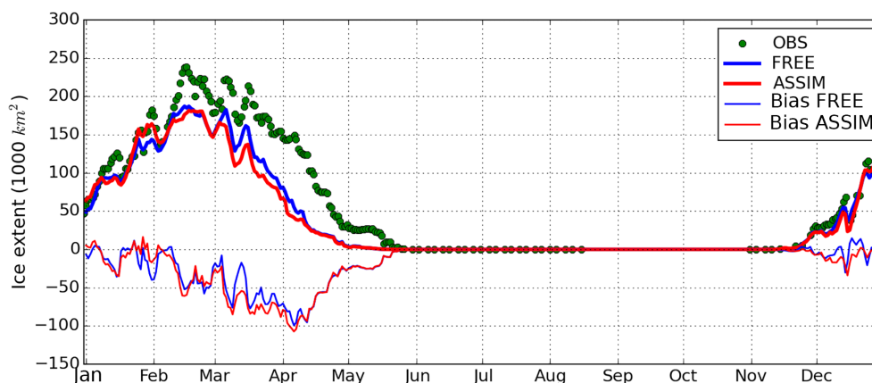
Figure 13. The daily sea-ice extent from FREE, ASSIM and IceMap, and the sea-ice extent bias (modeled minus observed field), respectively.
