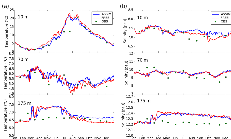
Figure 6. The time series of temperature (a) and salinity (b) at the BY15 station (57.33° N, 20.05° E) at depths of 10, 70 and 175 m, respectively.
