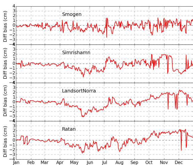
Figure 11. The variation of SLA biases in ASSIM relative to FREE against observations as a function of time. The station positions are shown in Fig. 8b.
