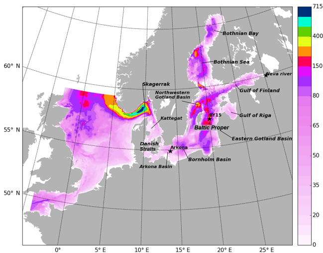
Figure 1. Geographical domain and bathymetry (in meters) of the NEMO-Nordic configuration.
