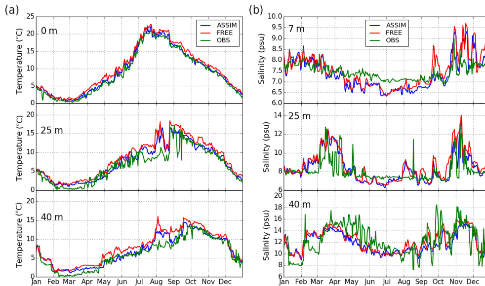
Figure 5. The time series of temperature (a) at depths of 0, 25 and 40 m and salinity (b) at depths of 7, 25 and 40 m at the Arkona station (54.88° N, 13.87° E), respectively.
