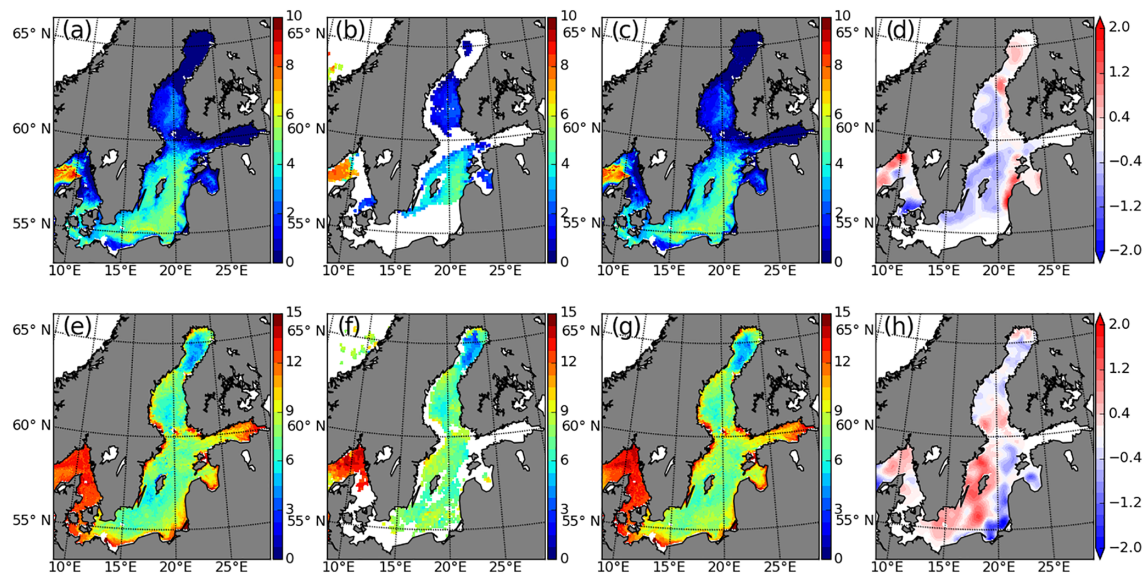
Figure 2. Map of SST from FREE (a, e), OSISAF (b, f), ASSIM (c, g) and the assimilation increments (d, h) on 11 January 2010 (a–d) and 2 June 2010 (e–h), respectively.
