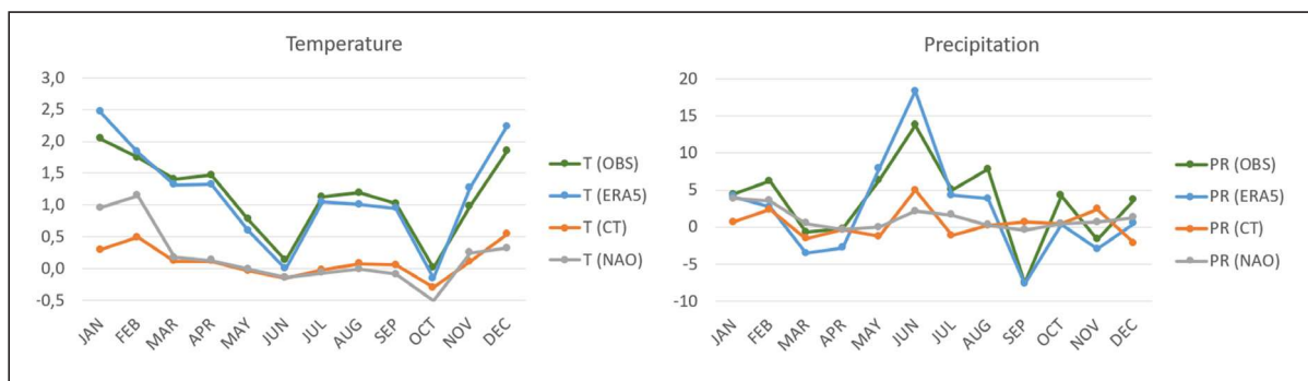
Figure 10 Changes in Swedish mean temperature (left, °C) and precipitation (right, mm/month) between 1961–1990 and 1991–2020. Observations (green) are from the SMHI data, reanalysis (blue) from ERA5. The synthetic temperature and precipitation series are derived from changes in the NAO-index (grey) and the analysis of circulation types (orange). See text.
