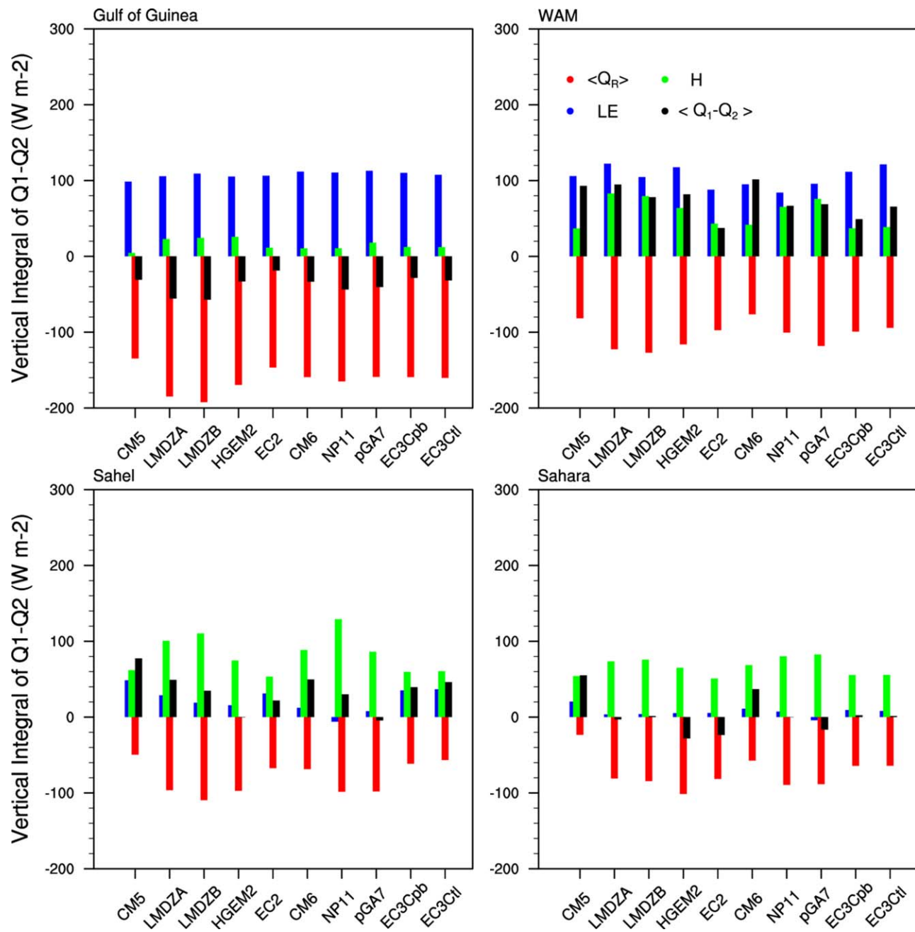
Figure 14. Vertically integrated Q_1 minus Q_2 (black) and the contributions from different physical processes, for the four key areas (W m -2 ). Contributions from: radiation (red), surface latent heat fluxes (blue), sensible heat fluxes (green). Note that partitioning by each model configuration within these broad definitions may not be exactly the same; therefore, these results are for overview purposes only.
