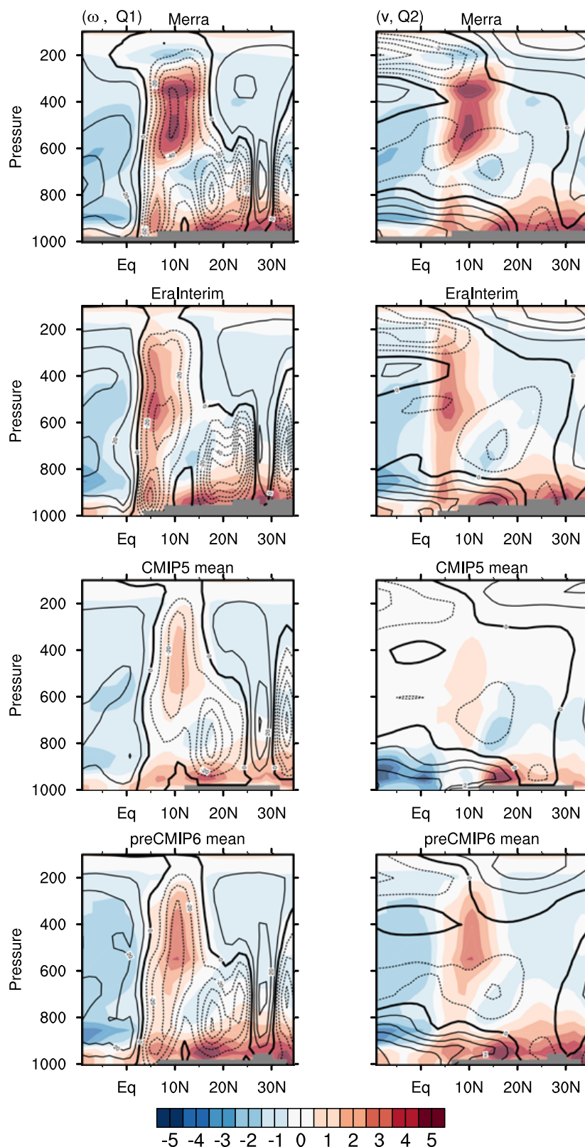
Figure 5. Latitudinal cross sections in JJA (10°W–10°E) of (left) Q_1 (diabatic heating) in \text{K d}^{-1} (colored shading) and pressure velocity in \text{hPa d}^{-1} (contour every 10 \text{hPa d}^{-1} , negative values with dotted lines) and (right) Q_2 (the effective heating due to drying from diabatic processes) in \text{K d}^{-1} (colored shading) and meridional wind in \text{m s}^{-1} (contour every 0.5 \text{m s}^{-1} , negative values with dotted line) for the African monsoon region, derived by the residual method from MERRA, ERA-I, and averages over the prototype-CMIP6 and CMIP5 model simulations.
