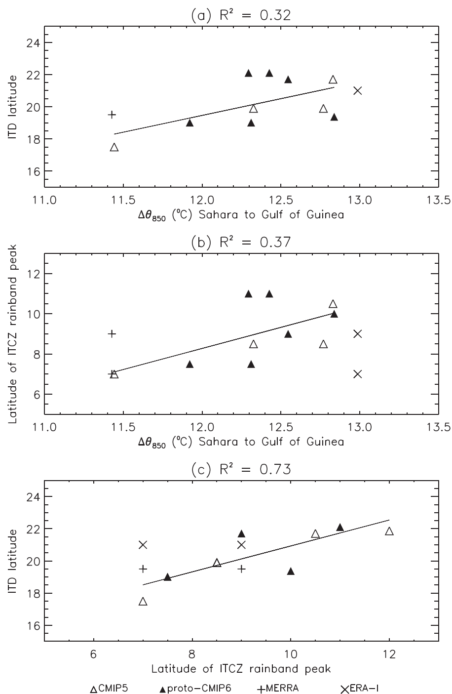
Figure 4. Scatter-plots showing the relationship between horizontal gradient in \theta_{850} between the Sahara and the Gulf of Guinea (defined as the difference between the box averages over the regions [10^{\circ}\text{W}-10^{\circ}\text{E}, 20-30^{\circ}\text{N}] and [10^{\circ}\text{W}-7^{\circ}\text{E}, 5^{\circ}\text{S}-3^{\circ}\text{N}] ) and: (a) the latitude of the ITD as determined from the location of the sign reversal of 10 m meridional winds averaged between 10^{\circ}\text{W} and 10^{\circ}\text{E} ; (b) the location of the WAM rainband peak. (c) The relationship between the ITD and ITCZ rainband peak latitudes. Regressions are taken over the model values only as the reanalyses and satellite rainfall observations may not be consistent.
