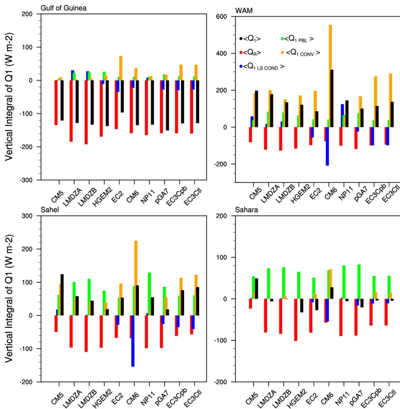
Figure 12. Vertically integrated Q_1 and the contributions from different physical processes, for the four key areas ( \text{W m}^{-2} ). Contributions from: radiation (red), large-scale condensation (blue), convection (orange), boundary layer mixing (green). Note the variation in scale of the vertical axes. Note also that partitioning by each model configuration within these broad definitions may not be exactly the same; therefore, these results are for overview purposes only.
