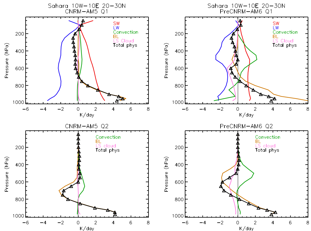
Figure 11. Q_1 and Q_2 components from different diabatic heating sources in the Saharan region ( 10^\circ\text{W} – 10^\circ\text{E} , 20^\circ\text{N} – 30^\circ\text{N} ) from CNRM-AM5 and PreCNRM-AM6.
