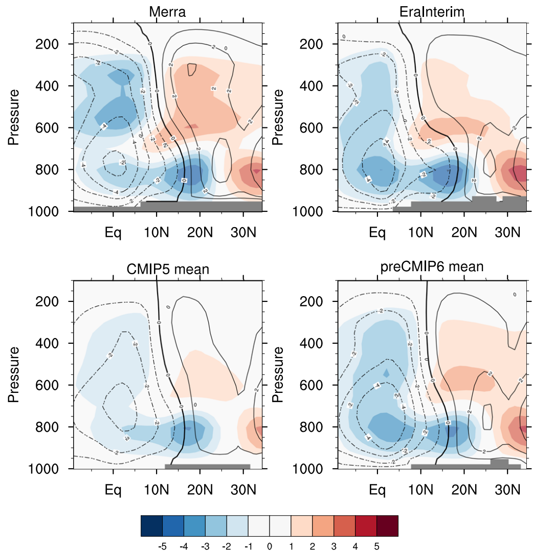
Figure 6. Meridional cross section of the ( 10^{\circ}\text{W} – 10^{\circ}\text{E} ) zonal mean mass stream function which balances Q_1 , (\overline{\psi^{nd}}) , colors) and nondivergent mass stream function \psi^{nd} (contours at same intervals as color scale, negative contours dotted) for JJA, in the two reanalyses and averaged over the CMIP5 and prototype-CMIP6 model simulations. Units are 10^{11} \text{ kg s}^{-1} .
