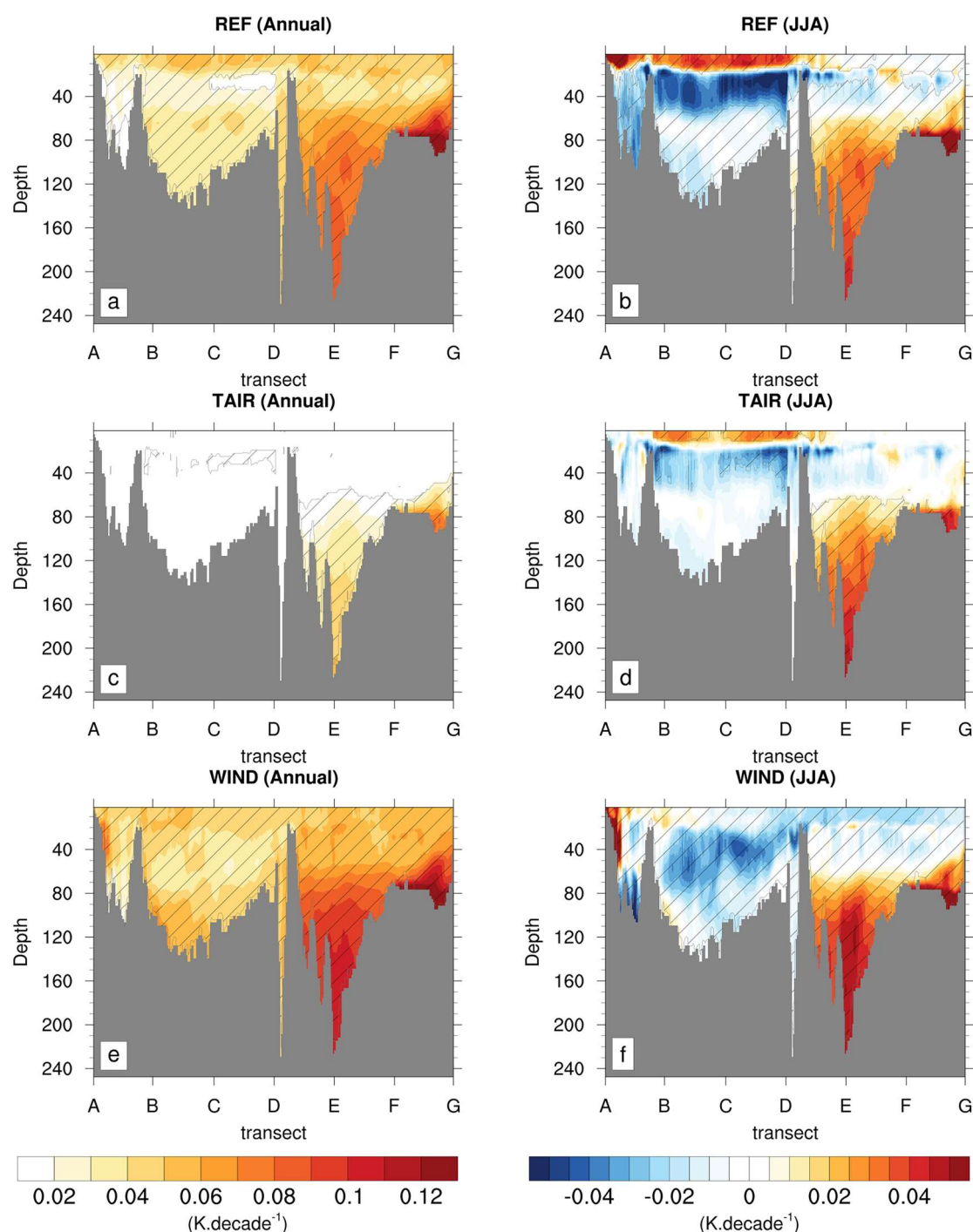
Fig. 12 Annual temperature trends and relative summer temperature trends (in \text{K decade}^{-1} ) computed over the 1850–2008 period (calculated as the seasonal SST trend minus the spatially averaged annual temperature trend). a, c, e Annual, b, d, f JJA. The temperature
