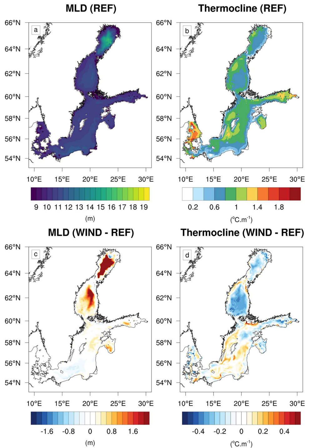
Fig. 13 Summer (JJA) mixed layer depth (MLD; in m) and maximum of thermocline strength (in ^{\circ}\text{C m}^{-1} ) (a–b) in REF and (c–d) difference between WIND and REF. See the "Method" section for the calculation of MLD and thermocline strength
