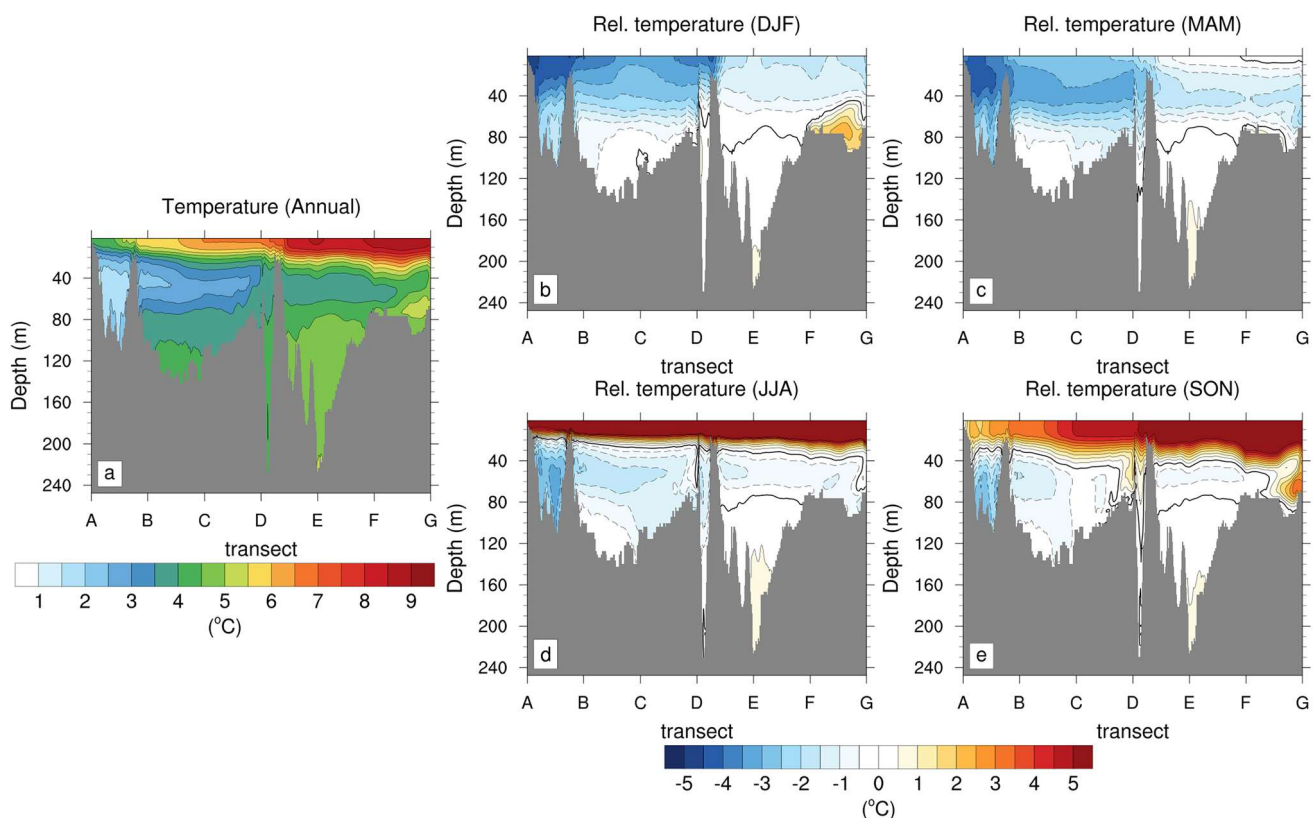
Fig. 4 Vertical transect of annual temperature and relative seasonal temperature (in ^{\circ}\text{C} ) from North to South of the Baltic Sea computed over the 1850–2008 period (calculated as the seasonal temperature minus the spatially averaged annual temperature). a Annual, b DJF,
