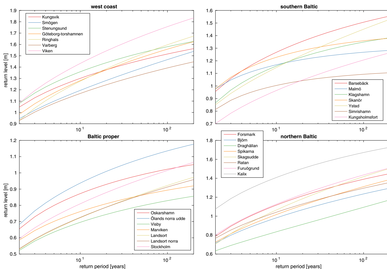
Fig. 5 Return level as a function of return period for the different stations. The geographical areas are the same as in Fig. 2. The x-axis is logarithmic
