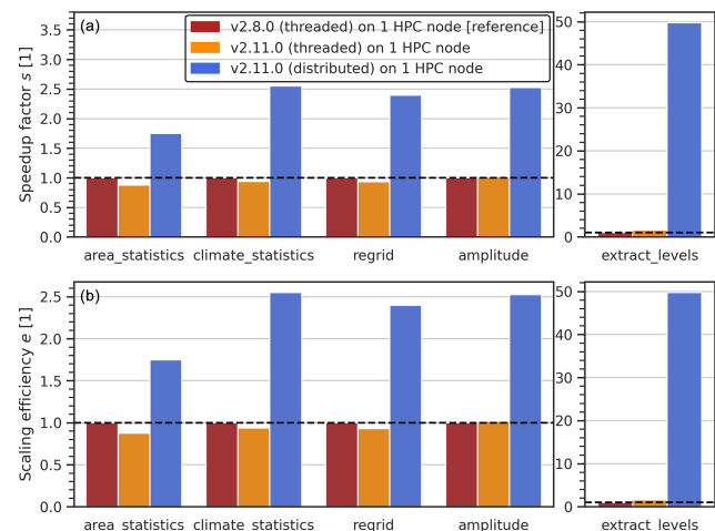
Figure 4. (a) Speedup factors (see Eq. 1) and (b) scaling efficiencies (see Eq. 2) of individual preprocessor runs in different setups (see legend). The speedup factors s and scaling efficiencies e are calculated relative to the reference setup. The input data are monthly-mean vertically resolved air temperature (time, pressure level, latitude, longitude) for 20 years of historical simulations (1995–2014) from 10 different CMIP6 models. The dashed black lines indicate no improvement relative to the reference setup, and values above/below these lines correspond to better/worse performance.
