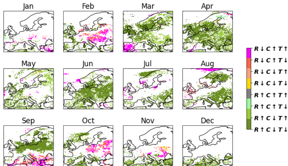
Figure 5. The climatic trend regimes based on the combination of trends in surface solar radiation ( R ), daytime cloud fraction ( C ), and liquid cloud optical thickness ( T ). The arrows show either an increasing or decreasing trend in these variables. The white areas show the regions with missing data or where the trends in either of them are not statistically significant.
