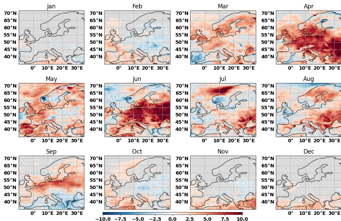
Figure 3. The spatial trends in SIS (in \text{W m}^{-2} per decade) based on the CLARA-A3 CDR (1982–2020). Only those trends that are significant at the 90 % confidence interval are shown.
