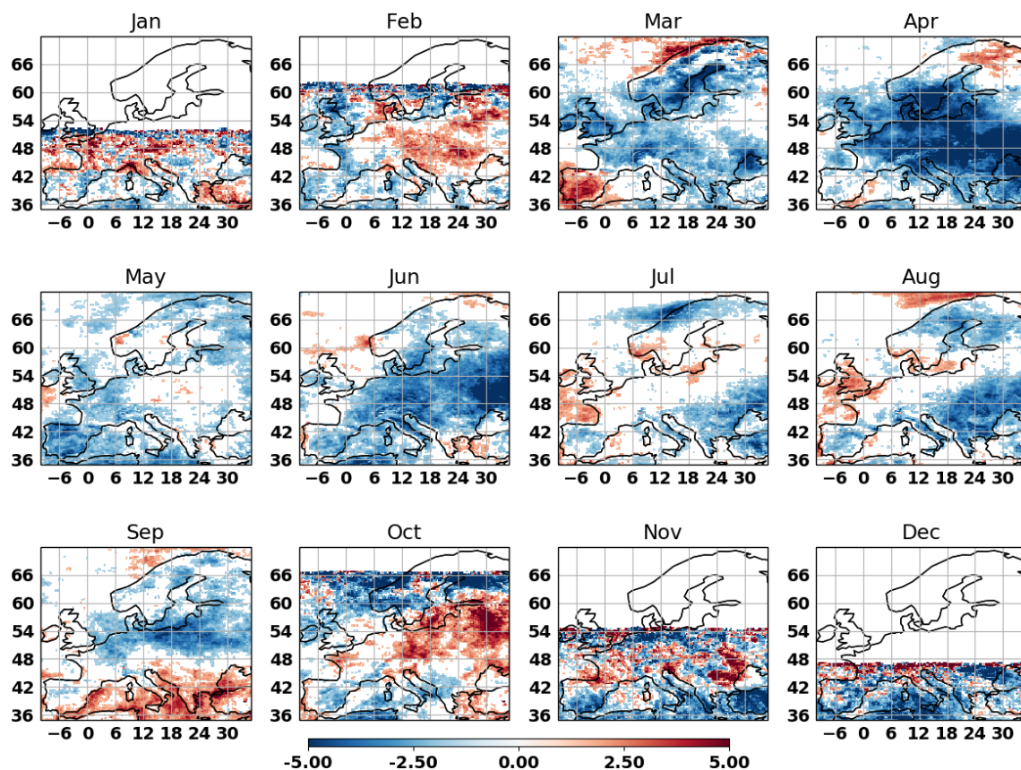
Figure 4. The spatial trends in daytime cloud fraction (in % per decade) based on the CLARA-A3 CDR (1982–2020). Only those trends that are significant at the 90 % confidence interval are shown.
