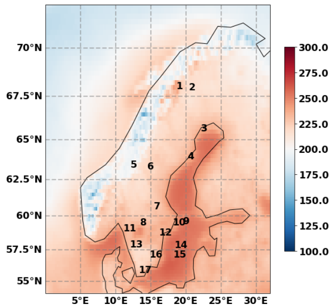
Figure 1. The geographical positions of 17 Swedish SIS measurement stations used to evaluate SIS monthly means in the CLARA-A3 CDR. The background shows climatological mean SIS (in \text{W m}^{-2} ) for the month of June (1991–2020) based on CLARA-A3.
