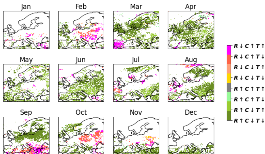
Figure 6. Same as in Fig. 5 but when ice cloud optical thickness is considered while deriving the climatic trend regimes.
