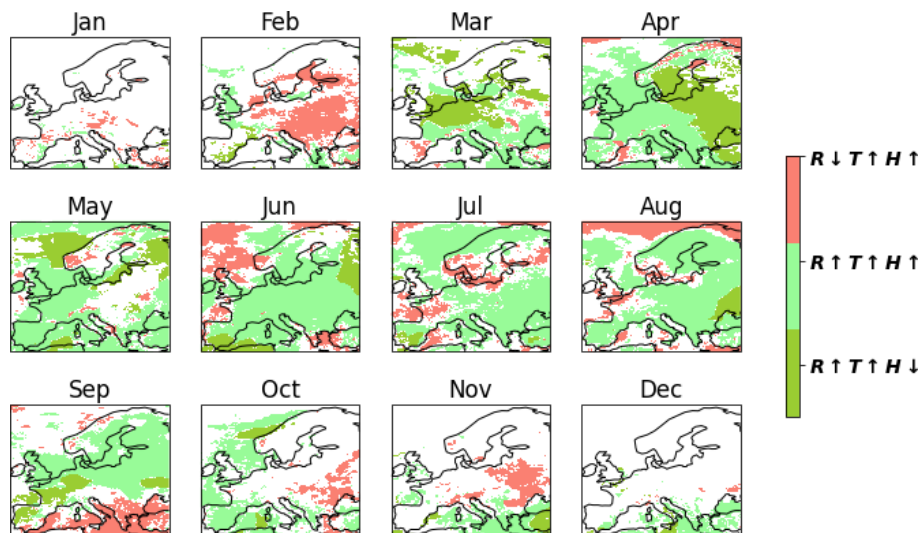
Figure 10. The interplay among trends in surface solar radiation ( R ), surface temperature ( T ), and total column water vapour ( H ). The arrows show either an increasing or decreasing trend in these variables. The white areas show the regions where the trend in either of them is not statistically significant.
