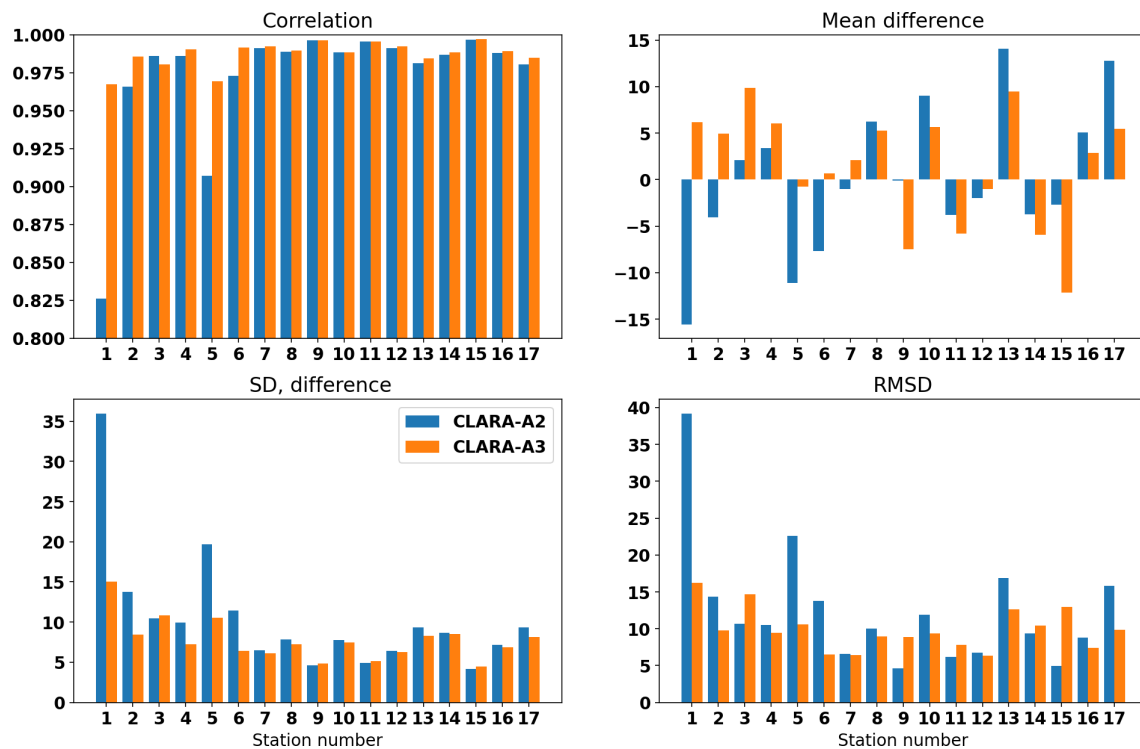
Figure 2. Evaluation of CLARA-A2 and CLARA-A3 SIS against the Swedish in situ measurements. The figures show the correlation coefficients, the mean difference, the standard deviation of the difference, and the root-mean-square difference. The units are in \text{W m}^{-2} .
