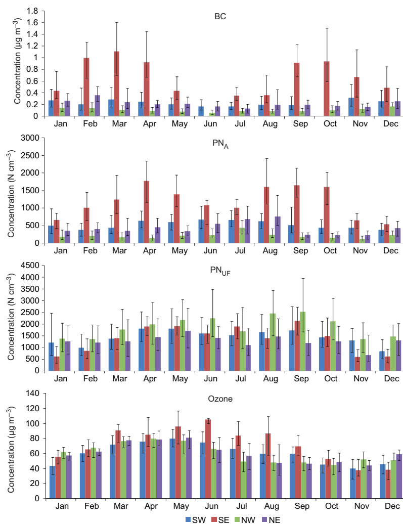
Fig. 6. Monthly median concentrations of BC, PN_A (accumulation mode number concentration), PN_{UF} (ultrafine mode particle number concentration) and daily maximum eight-hour mean ozone concentrations in the four sectors averaged over all available data in the period 1997–2010. Vertical bars are 75 and 25 percentiles.
