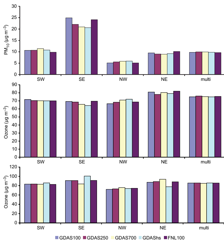
Fig. A2-1. Annual mean of PM_{10} (top); annual (middle), and March–September (bottom) means of daily maximum eight-hour ozone concentrations in air classified by sector based on trajectories from five sensitivity cases for 2005 (see Table A2-1).
