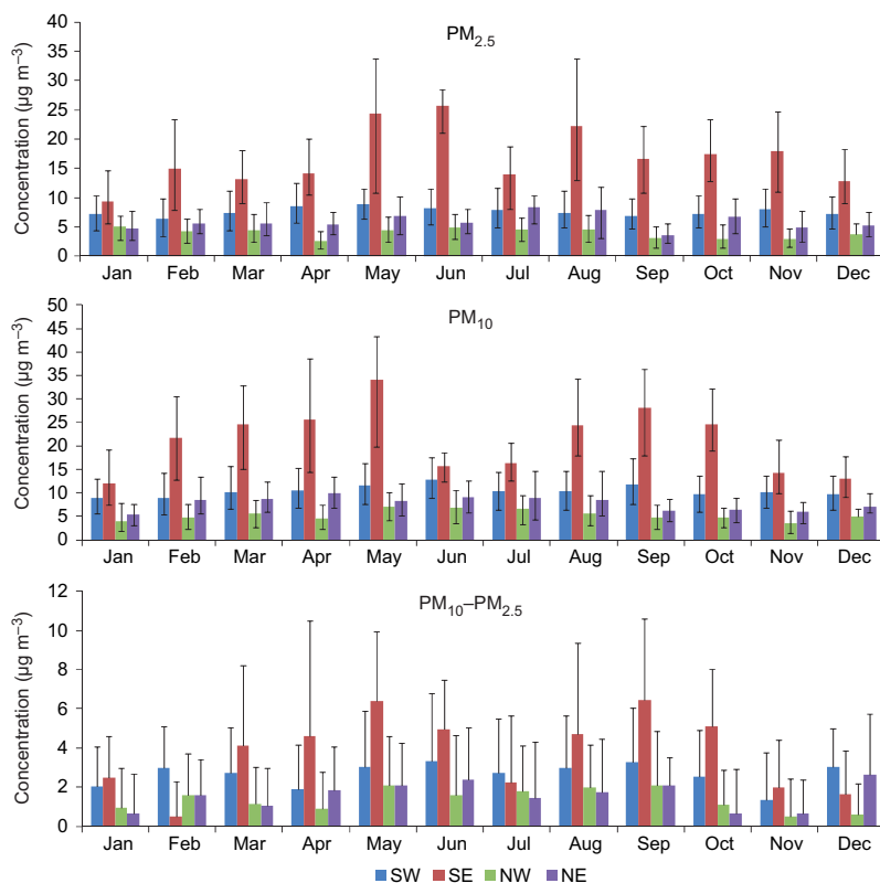
Fig. 5. Monthly median concentrations of PM 2.5 , PM 10 and PM 10 -PM 2.5 (coarse mode particulate matter) concentrations in the four sectors averaged over all available data in the period 1997–2010. Vertical bars are 75 and 25 percentiles.
