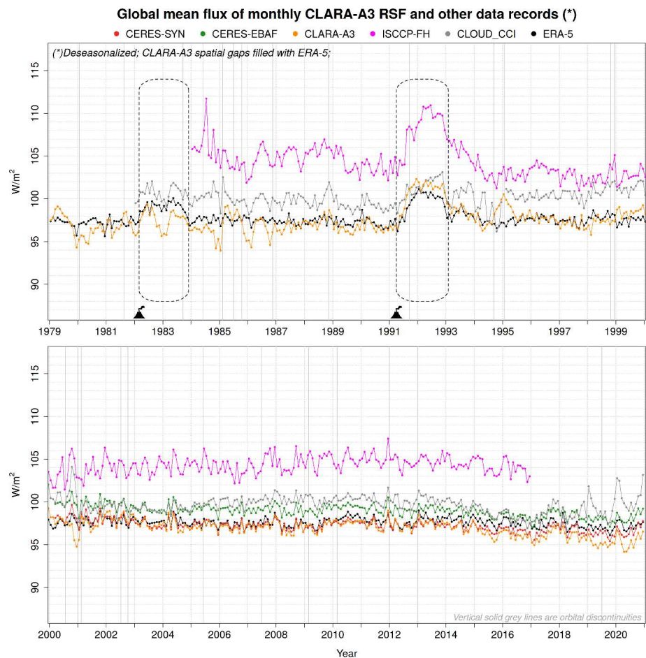
Figure 10. Global mean flux of monthly CLARA-A3 RSF and other data records. The periods with radiative impact from two major volcanic eruptions, El Chichón (March 1982–December 1983) and Pinatubo (April 1991–January 1993), are indicated.
