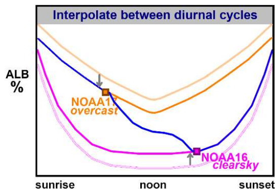
Figure 8. Conceptual illustration of the RSF temporal interpolation (figure not to scale). The average (expected) SZA–albedo curves associated with each observation’s scene type are shown in light colors (orange and pink). These curves are scaled to match the respective observations, which are shown in dark colors (orange and magenta). The final interpolated diurnal cycle is shown in blue.
