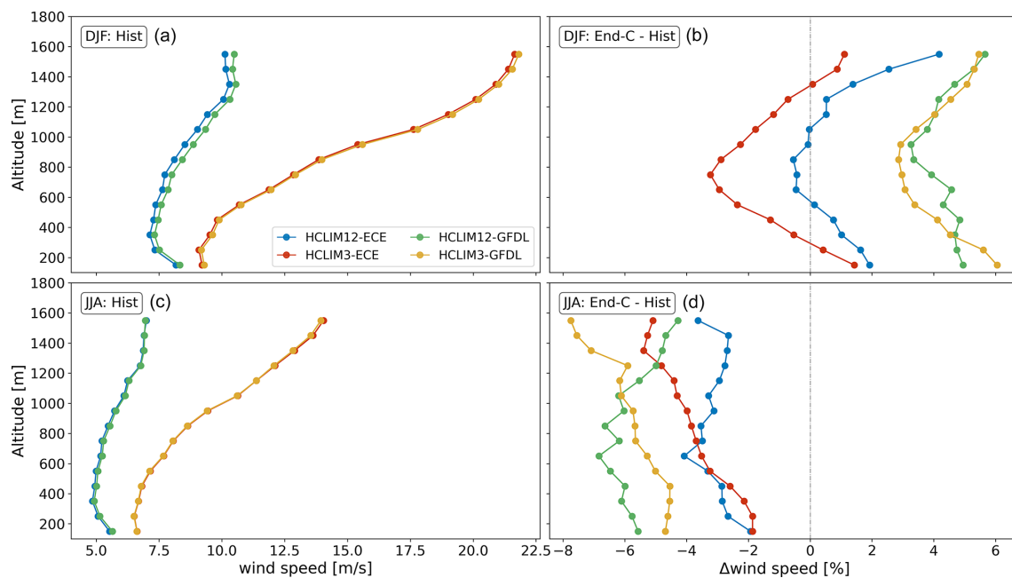
Figure 4. The 95th percentile of daily maximum 10m wind speed as a function of terrain height over the southern Norway subdomain (indicated in Fig. 2) in HCLIM3 and HCLIM12 scenarios for DJF (a, b) and JJA (c, d). Shown are the wind speeds in the historical period (a, c) and the change, in percent, by the end of the century (b, d). The data are bin-averaged over 15 vertical bins that are 100 m high.
